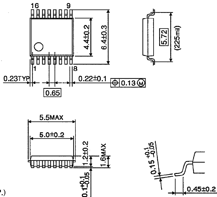
SSOP 16PIN OUTLINE DRAWING (SSOP16-P-225B)
