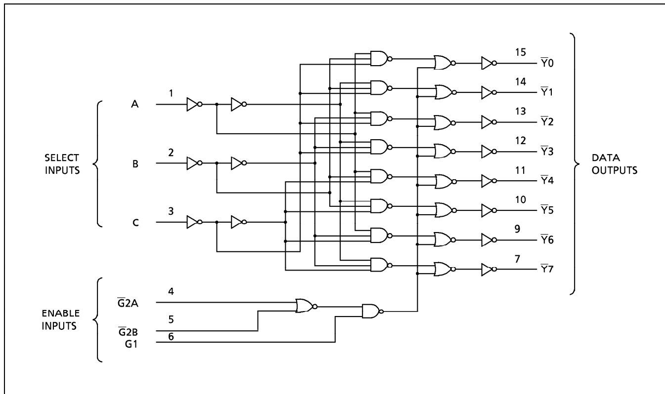
LOGIC DIAGRAM
