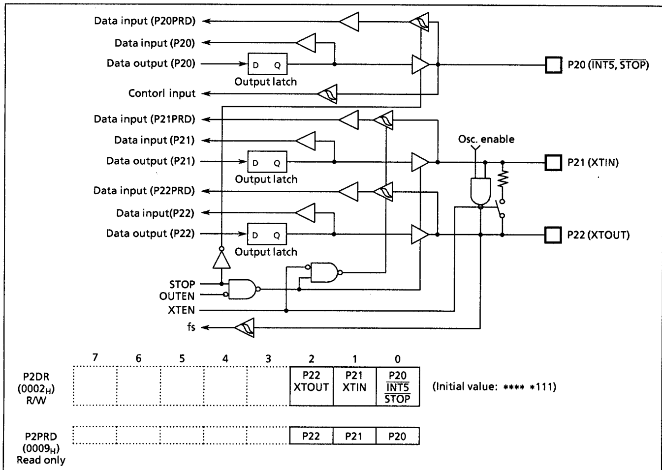
Figure 2-4. Port 2
