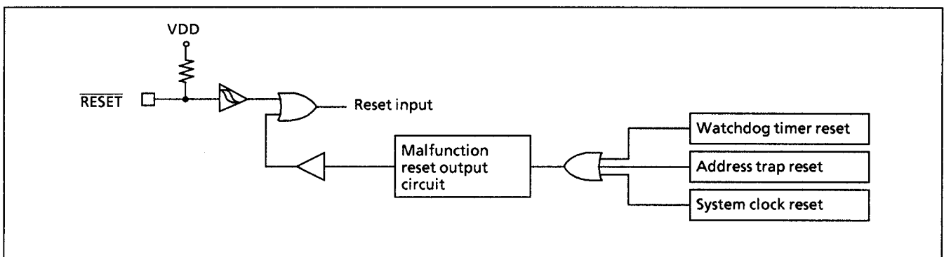
Figure 1-21. Reset Circuit
