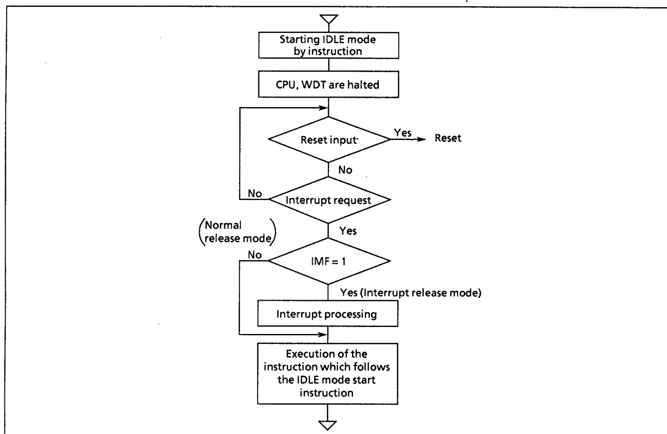
Figure 1-12. IDLE Mode
