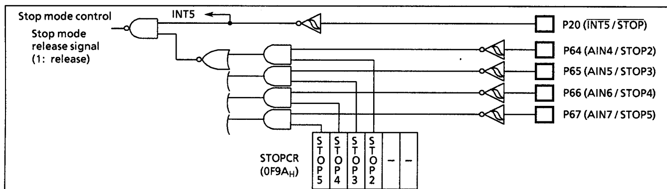
Figure 2-66. Stop Mode Control Circuit
