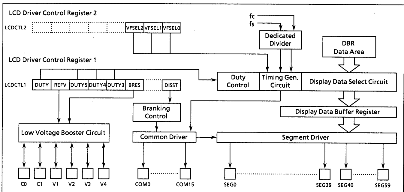
Figure 2-68. LCD Driver Block Diagram
