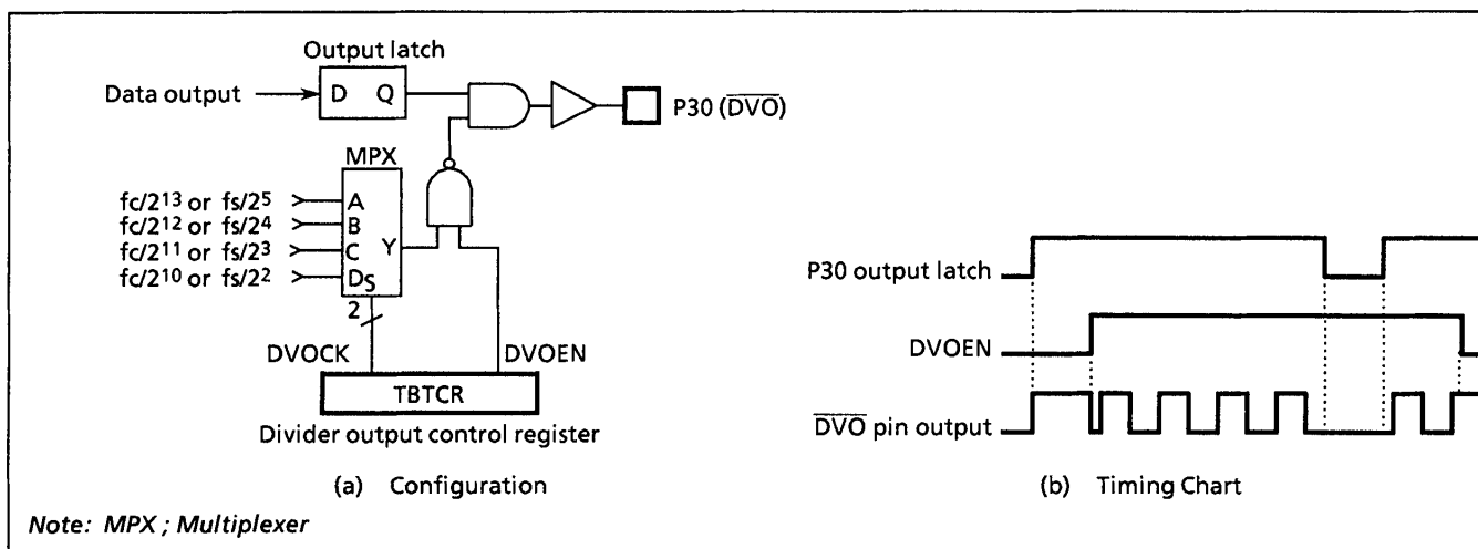
Figure 2-16. Divider Output
