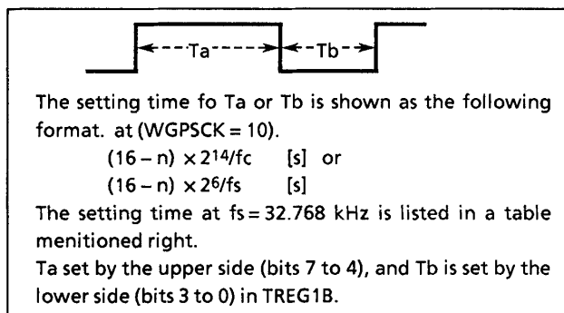
Figure 2-23. Window Gate Pulse Format
