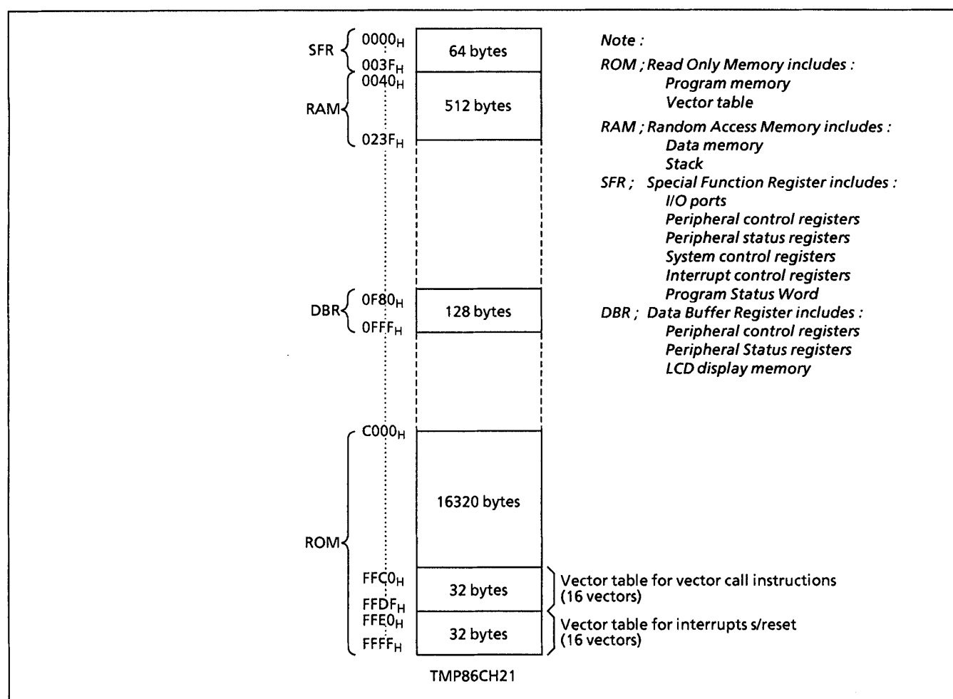
Figure 1-1. Memory Address Map
