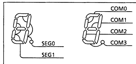
Figure 2-73. Example of COM, SEG Pin Connection (1/4 Duty)
