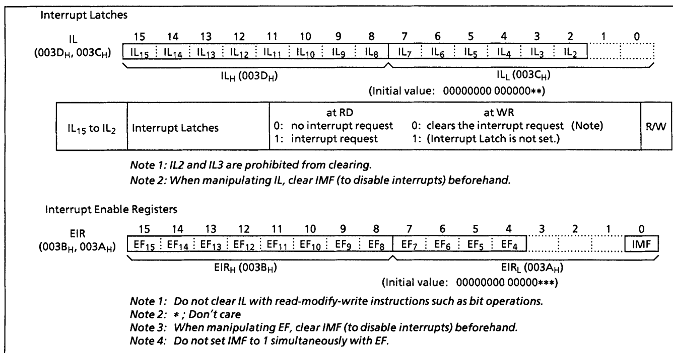
Figure 1-18. Interrupt Latch (IL), Interrupt Enable Registers (EIR)
