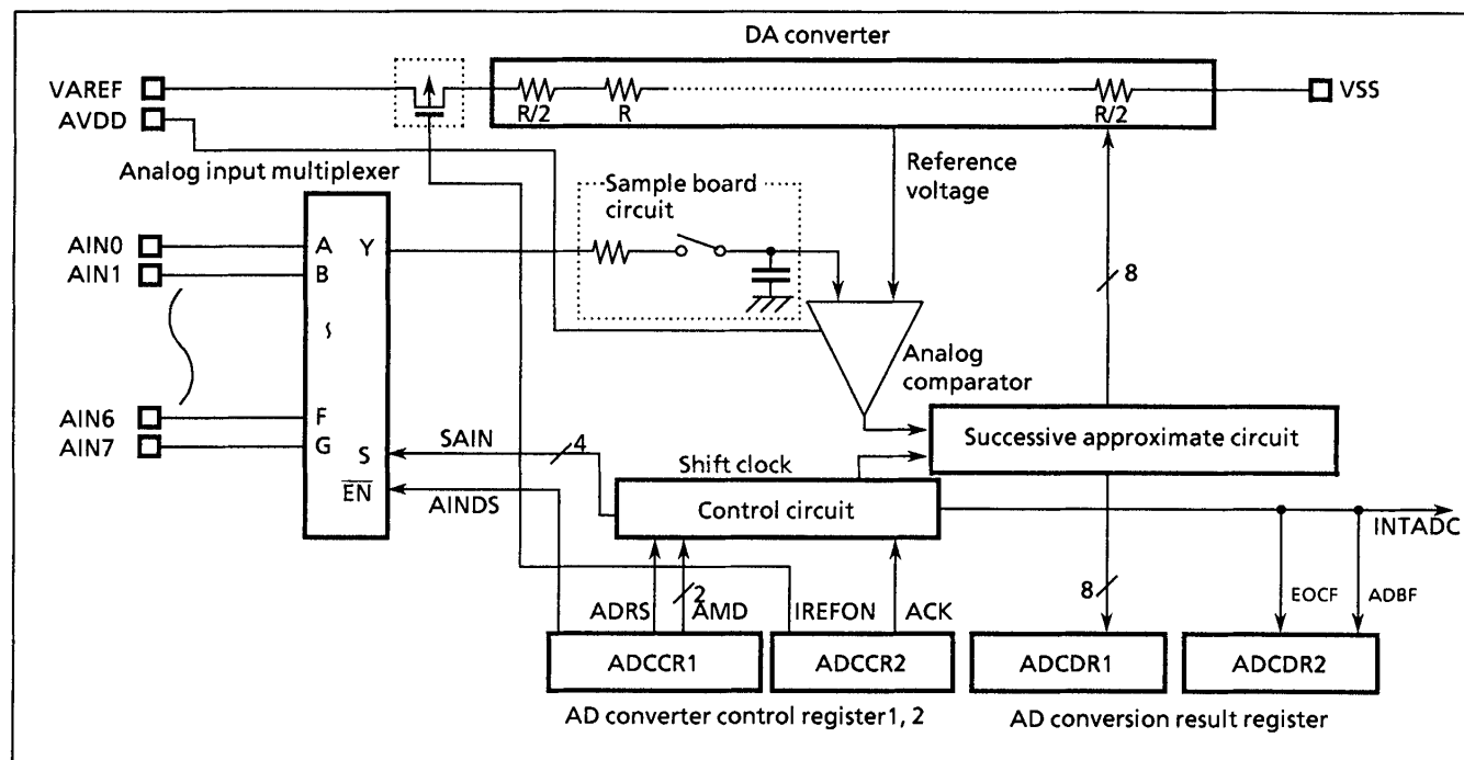
Figure 2-58. AD Converter (ADC)
