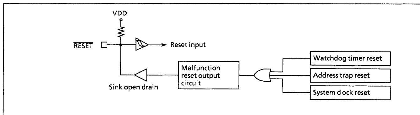
Figure 1-23. Reset Circuit
