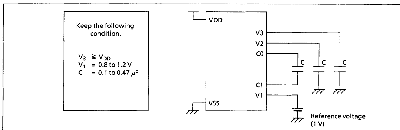
Figure 2-69. Example of a Booster Circuit (LCDCR<BRES> = "1")
