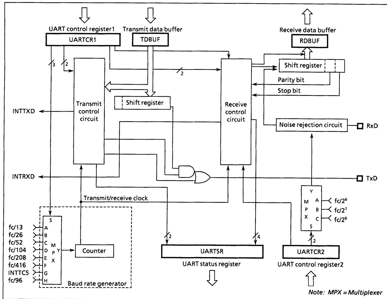
Figure 2-38. UART
