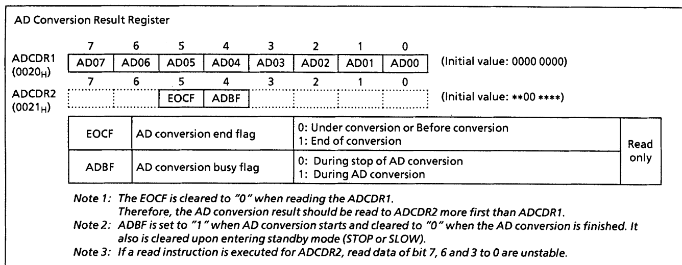
Figure 2-60. AD Converter Result Register
