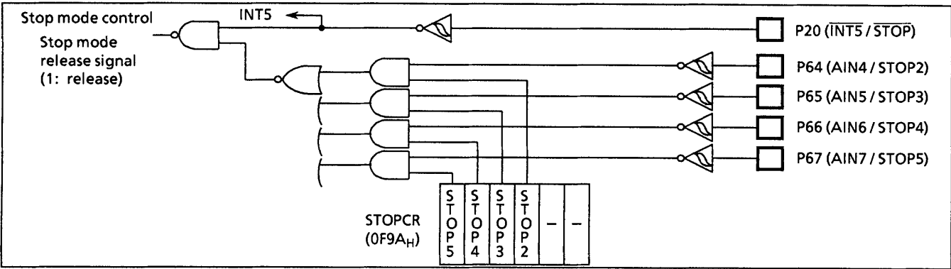
Figure 2-64. Stop Mode Control Circuit
