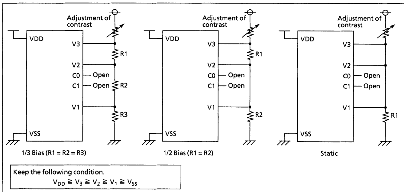
Figure 2-70. Example of Divider Resistance (LCDCR<BRES> = "0")
