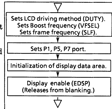
Figure 2-72. Initial Setting of LCD Driver
