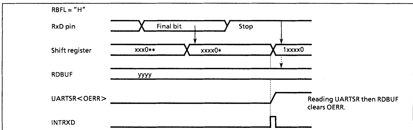
Figure 2-44. Generation of Overrun Error
