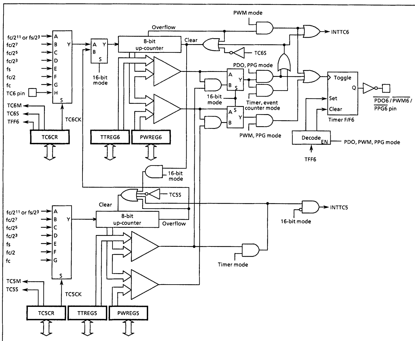
Figure 2-26. 8-Bit Timer 5, 6
