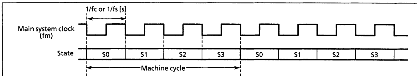
Figure 1-6. Machine Cycle
