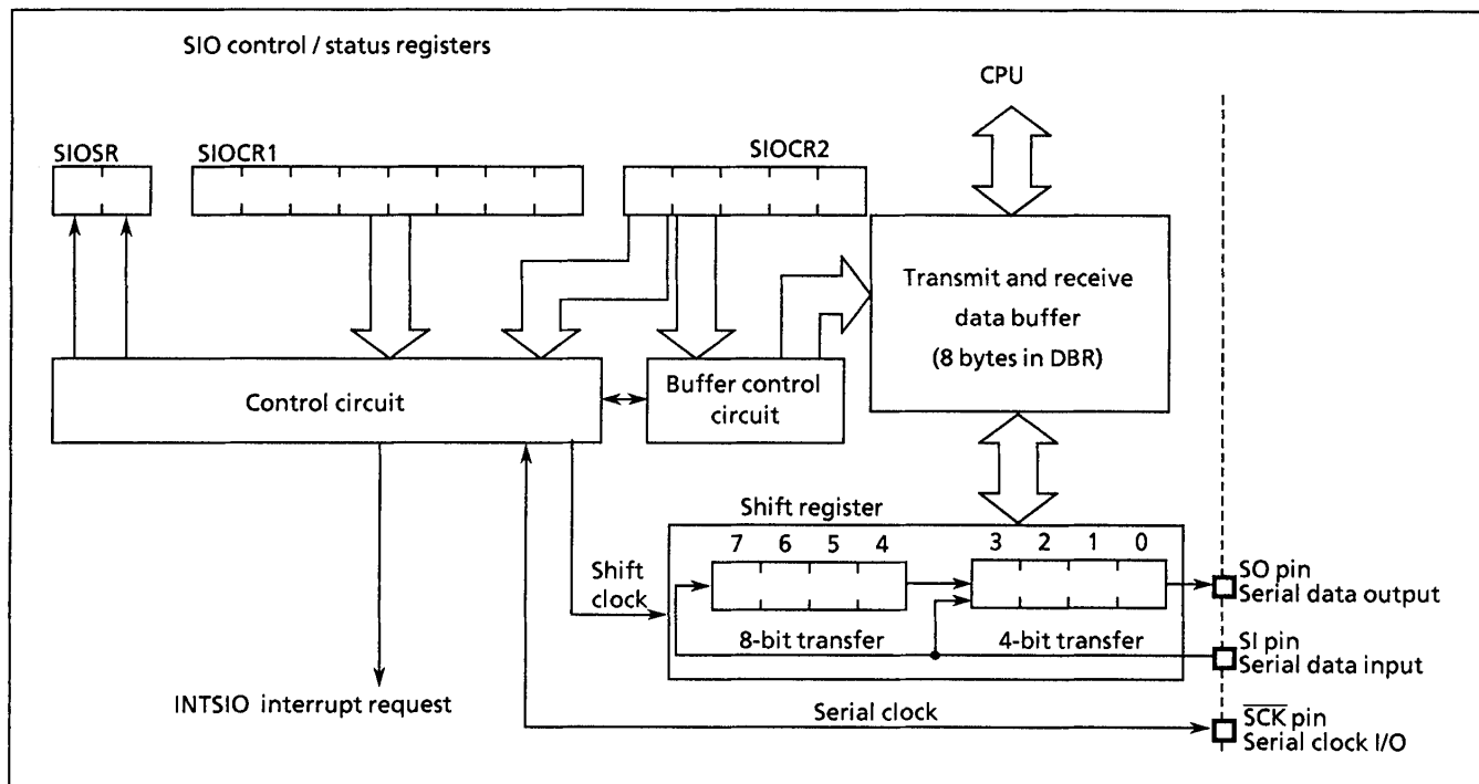
Figure 2-48. Serial Interfaces
