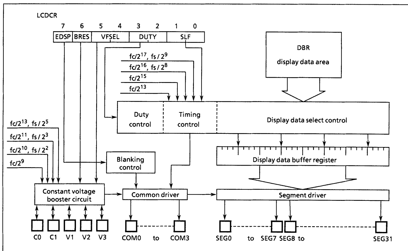
Figure 2-66. LCD Driver
