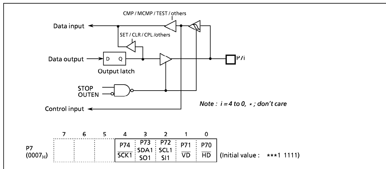
Figure 2-11. Port P7
