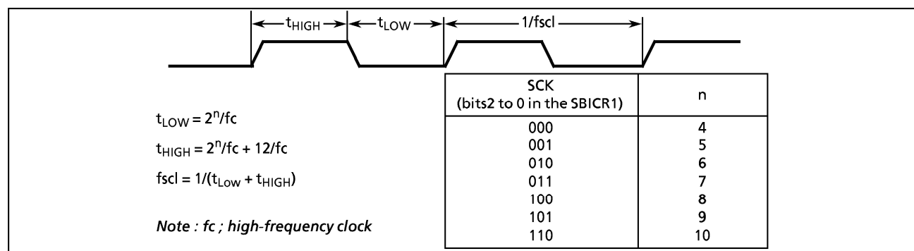
Figure 2-37. Clock Source
