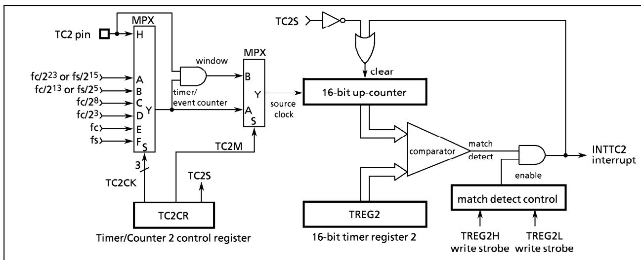
Figure 2-25. Timer / Counter 2 (TC2)
