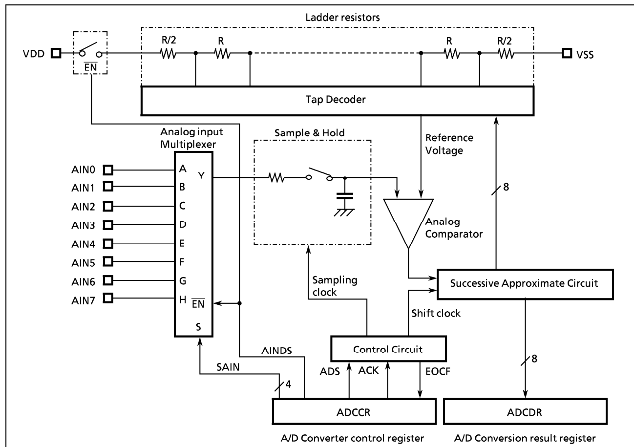
Figure 2-67. A/D Converter
