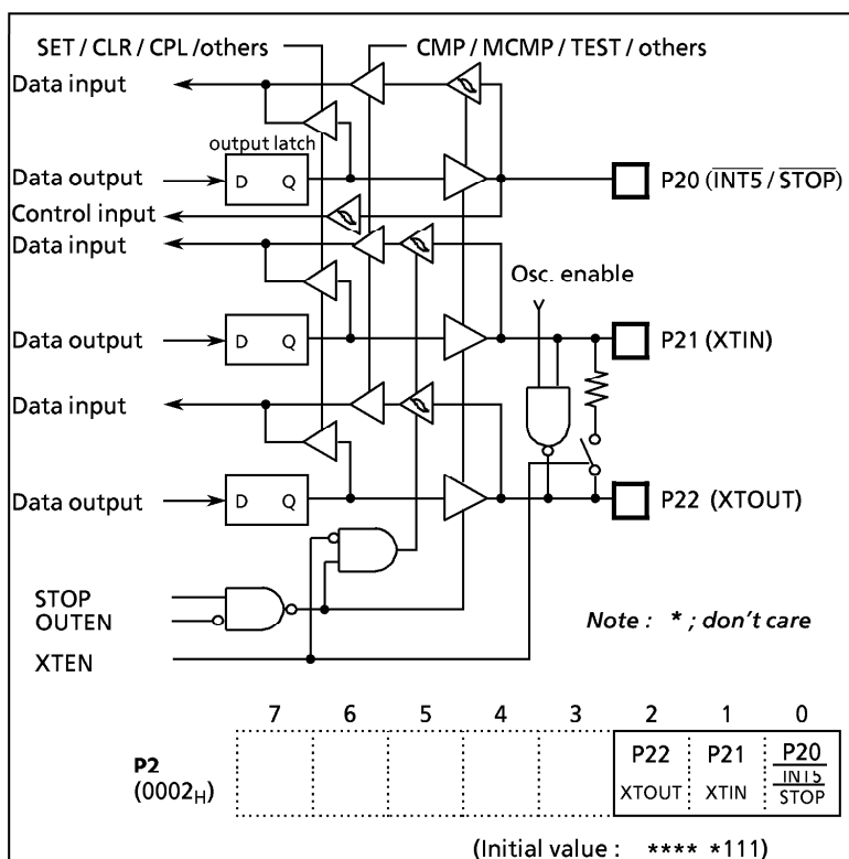
Figure 2-6. Port P2
