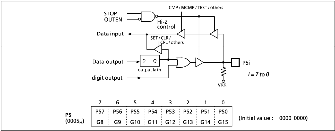
Figure 2-8. P5 Port
