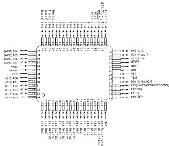
(2) QFP64-P-1420-1.00A
