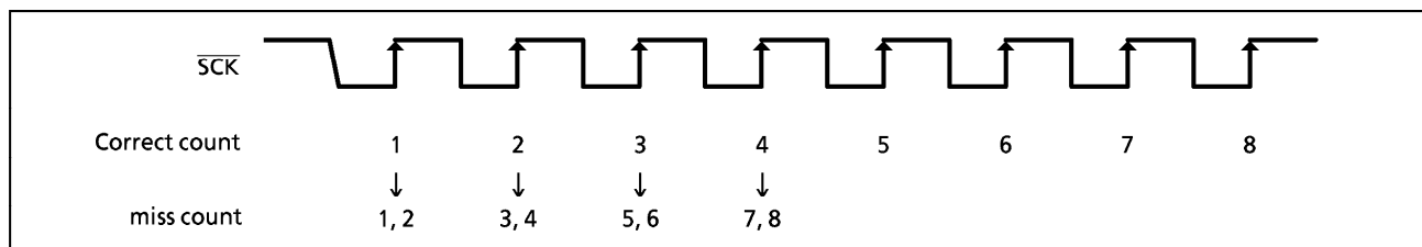
Figure 2. Example of miss count (at 8-bit receive mode)
