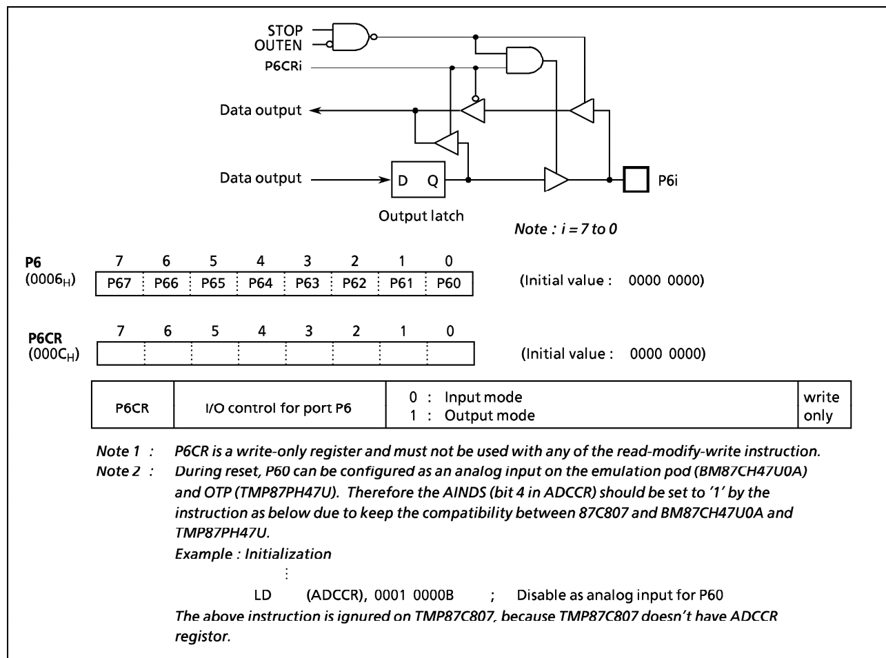
Figure 2-6. Port P6 and P6CR
