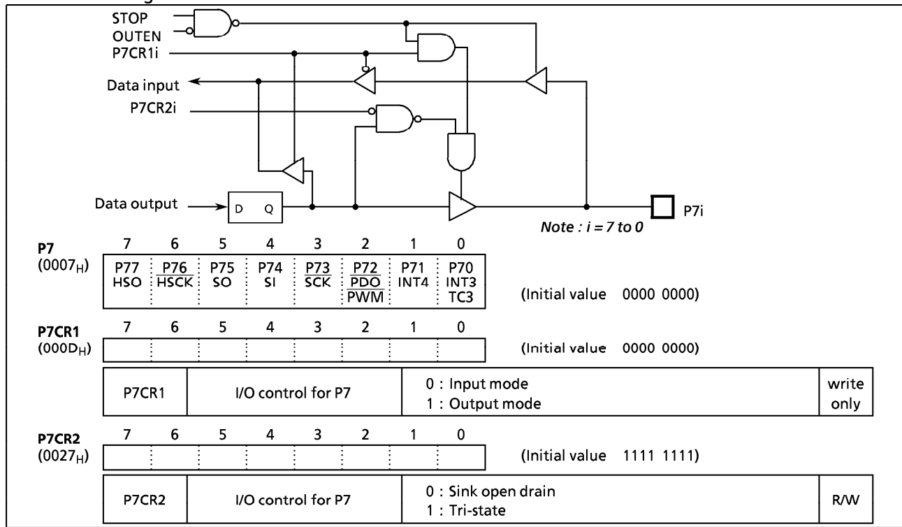
Figure 2-7. Port 7 and P7CR
