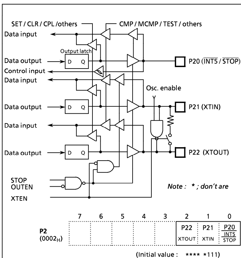
Figure 2-5. Port P2
