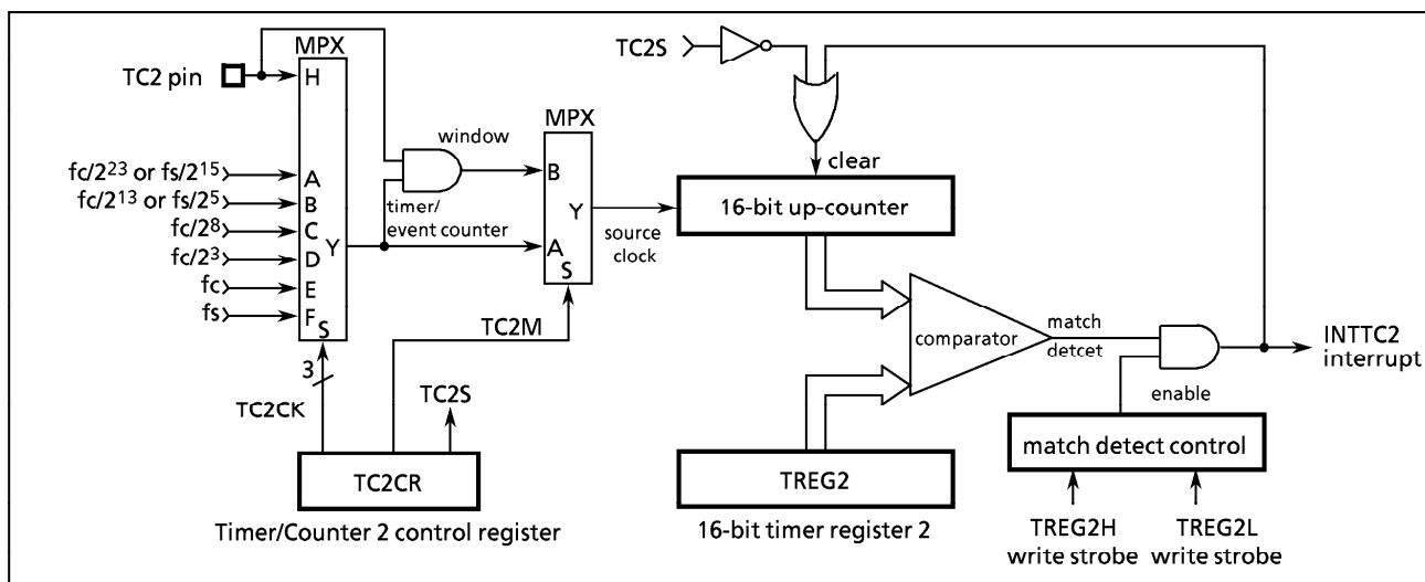
Figure 2-22. Timer/Counter 2 (TC2)
