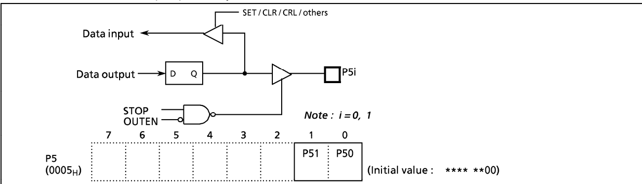
Figure 2-8. Port P5
