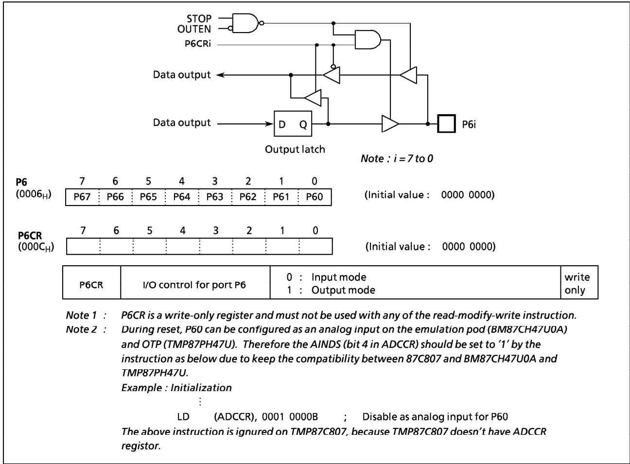
Figure 2-6. Port P6 and P6CR
