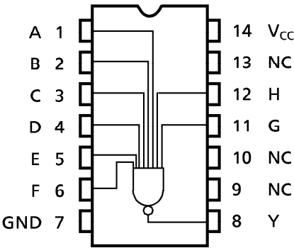
(TOP VIEW) NC : No Connection
