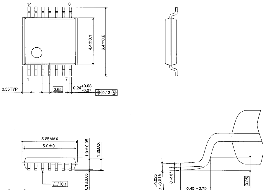
TSSOP 14PIN (170mil BODY) OUTLINE DRAWING (TSSOP14-P-0044-0.65) Unit in mm
