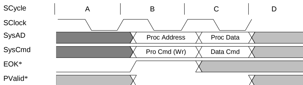
Figure 6.3.9 Sample Cycle with EOK* Asserted, Then Deasserted
