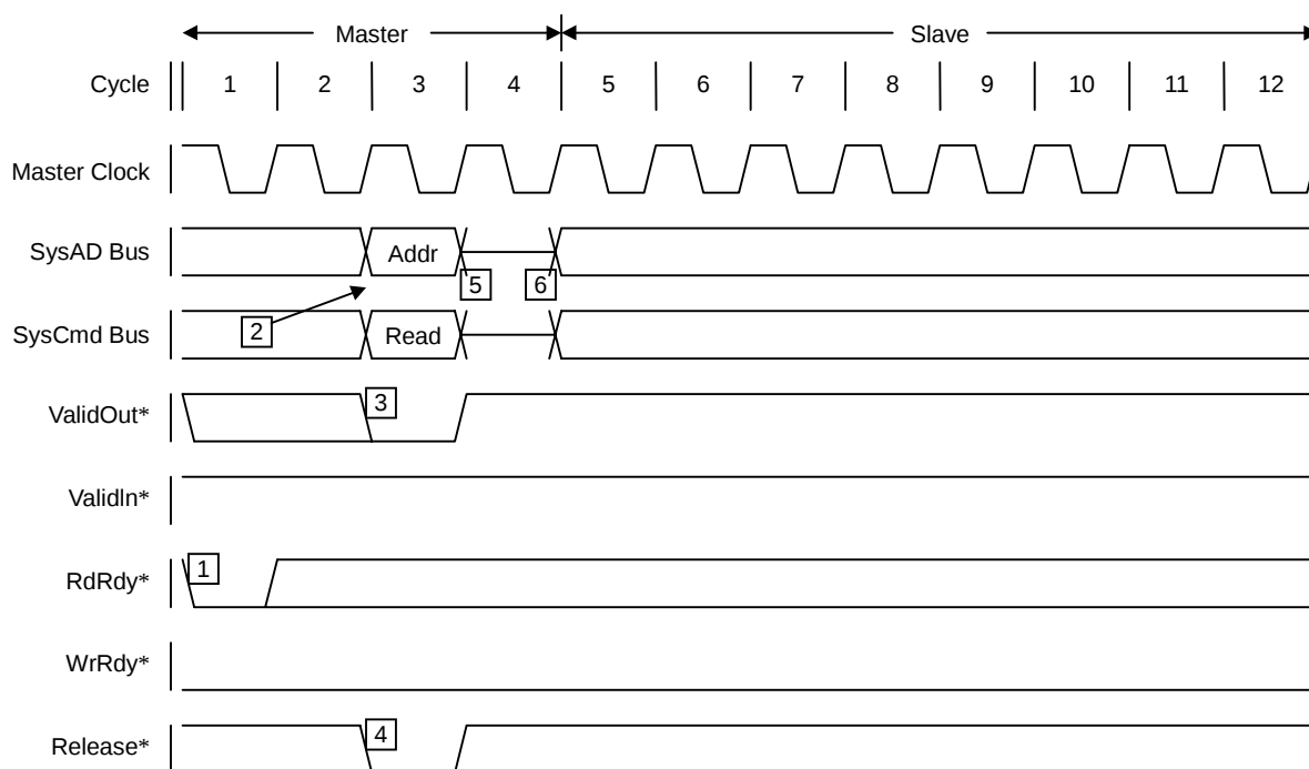
Figure 6.2.12 Processor Read Request Protocol
