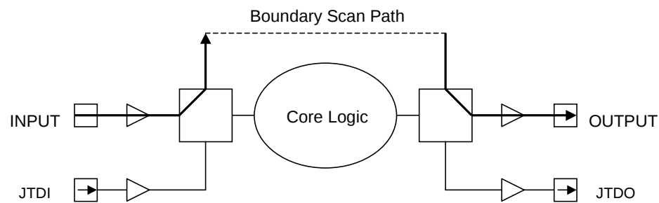
Figure 7.4.1 Test Data Flow While the EXTEST Instruction is Selected
