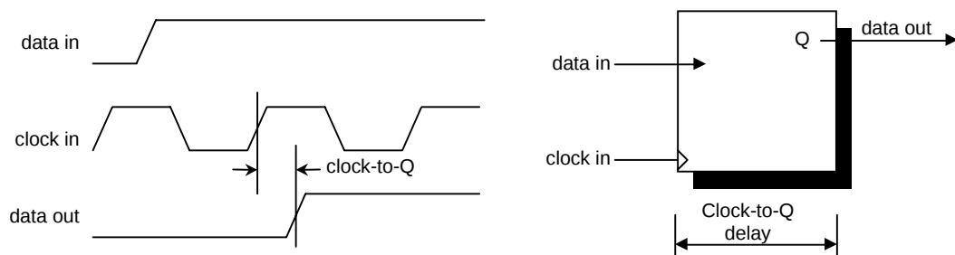
Figure 4.1.2 Clock-to-Q Delay
