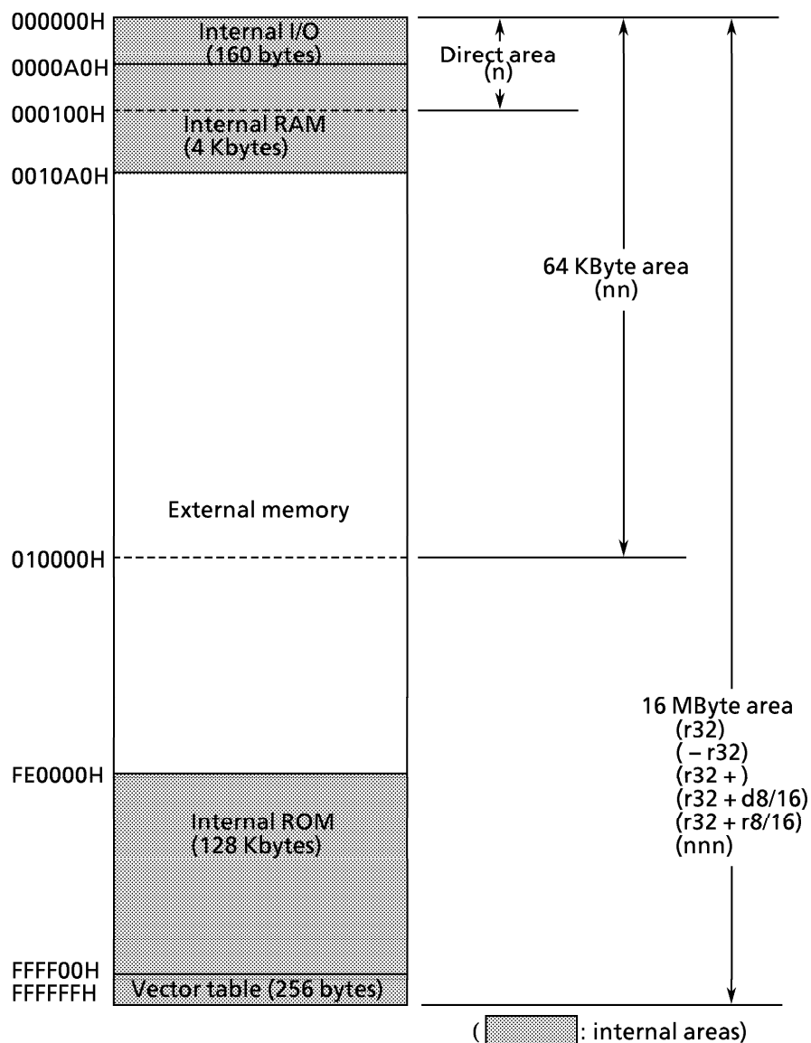
Figure 3.1 TMP95PW64 Memory Map
