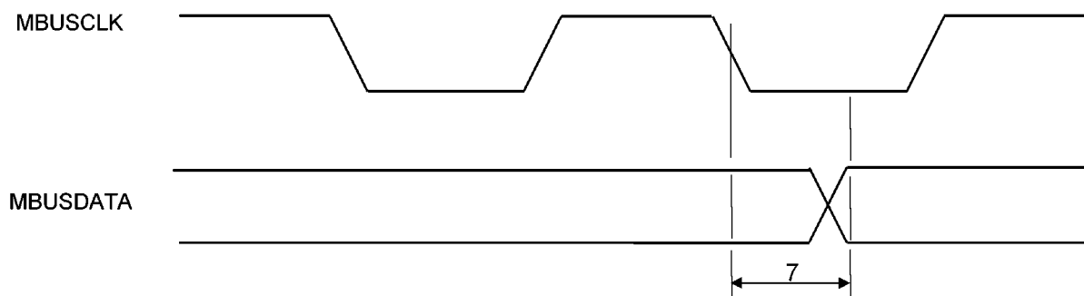
Magic Bus Output and Clock Timing (Master, PHAPOL=0)
