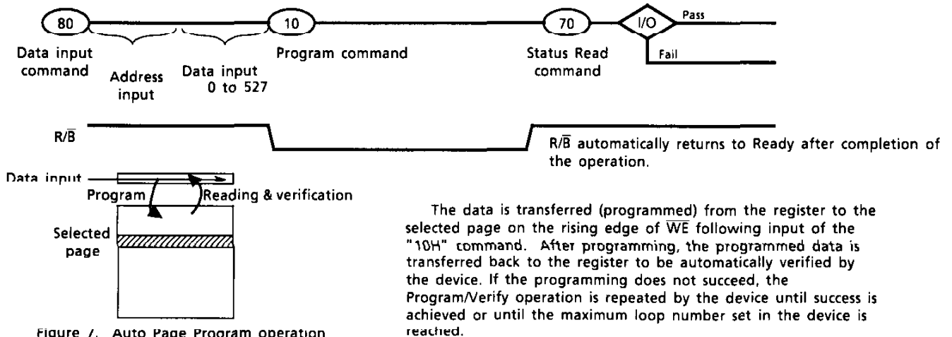
Figure 1. Auto Page Program operation
