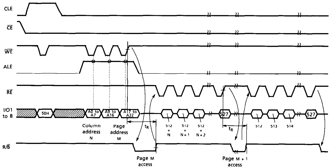
Sequential Read (3) Timing Diagram
