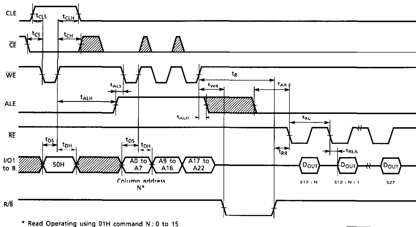
Read Cycle (3) Timing Diagram
