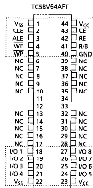
Figure 1. Pinout
