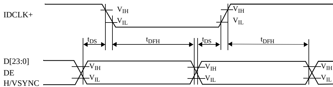
Dual-edge Clock to Data Setup/Hold timings
