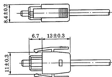
(1) Fiber optic connector
