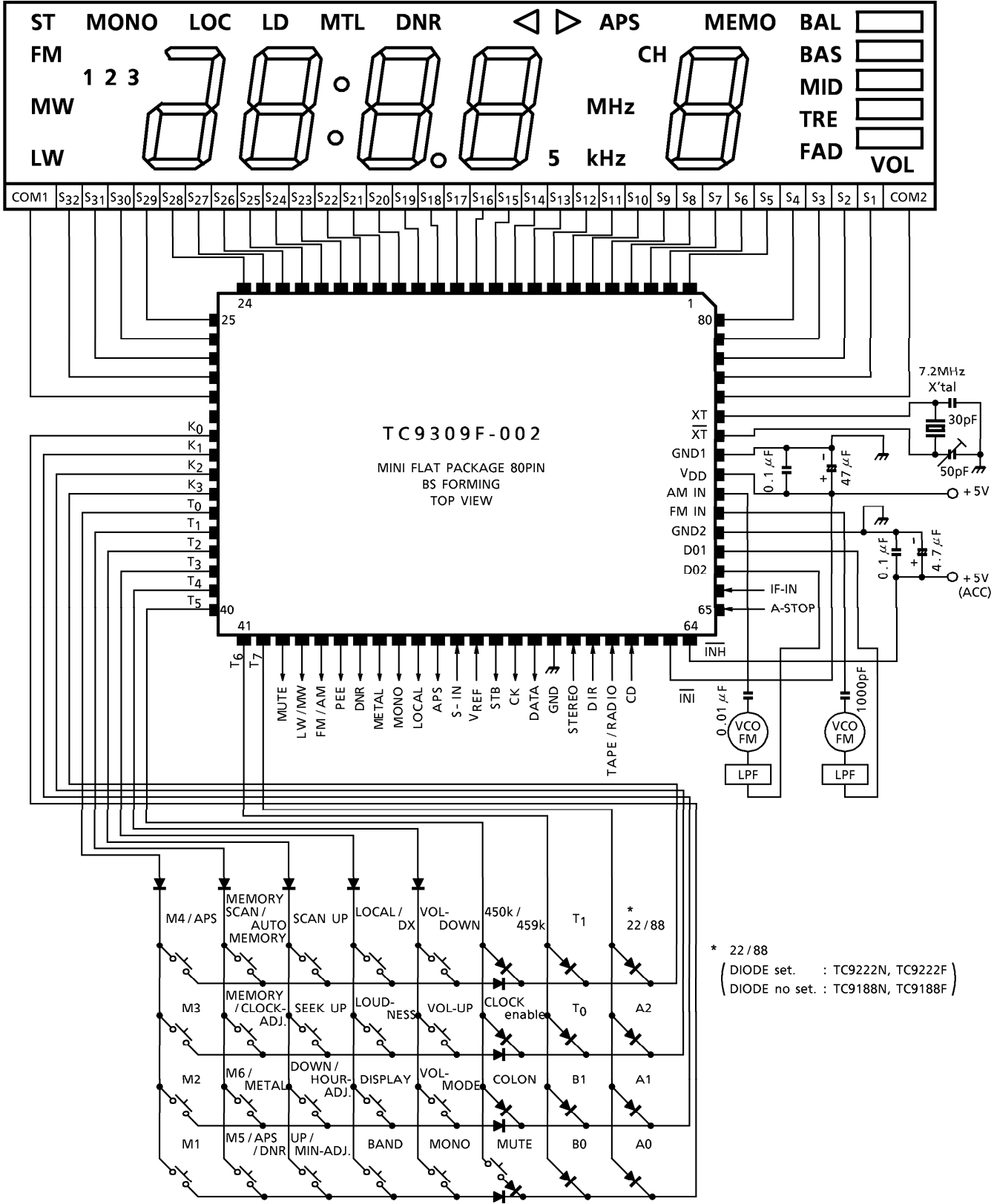
TC9309F-002 Layout
