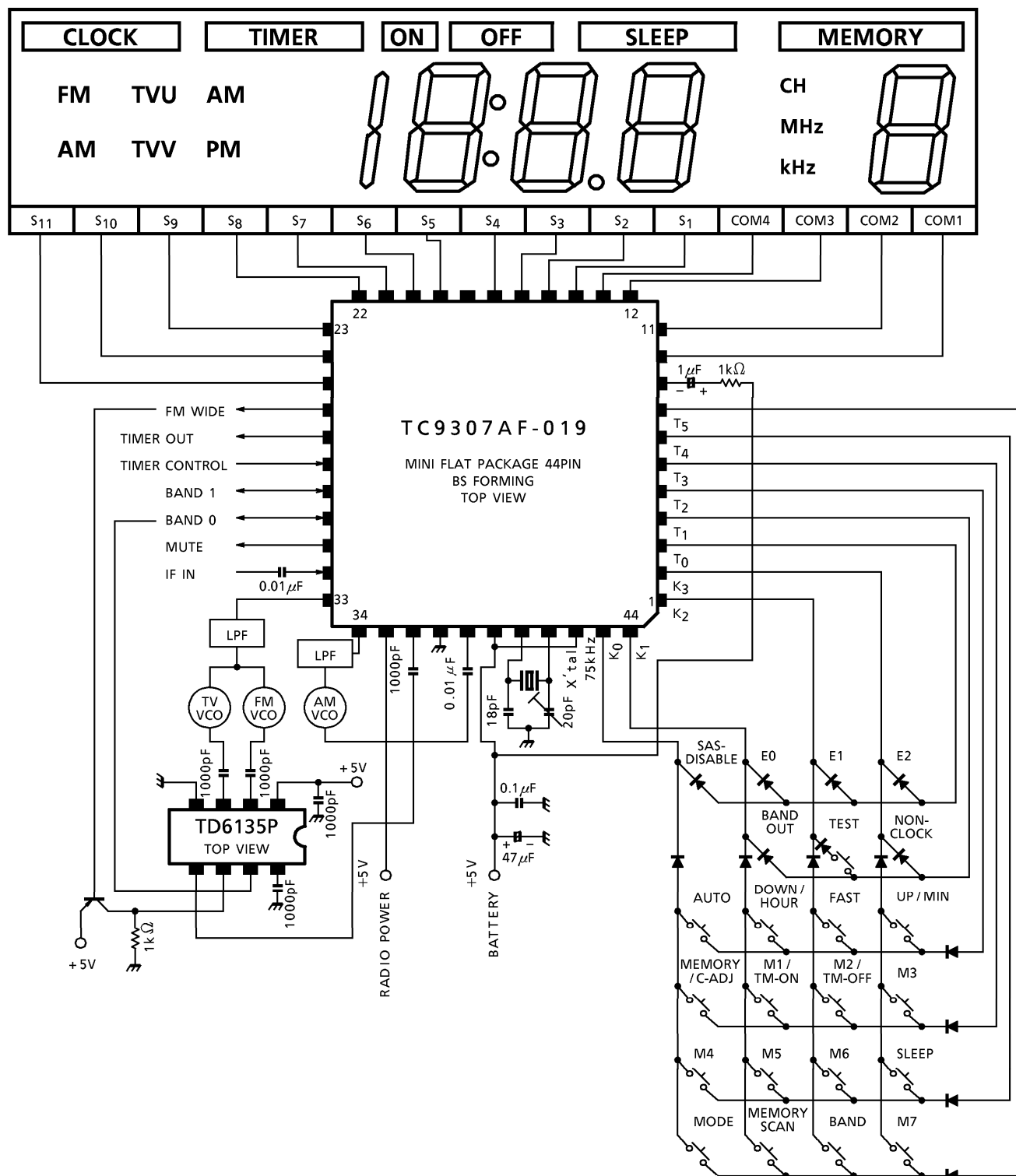
TC9307AF-019 Layout-4 (JAPAN area)
