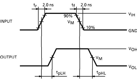
Fig.2 t_{pLH} , t_{pHL}
