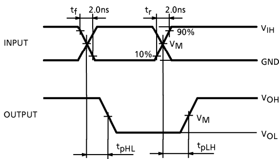
Fig.2 t_{pLH} , t_{pHL}
