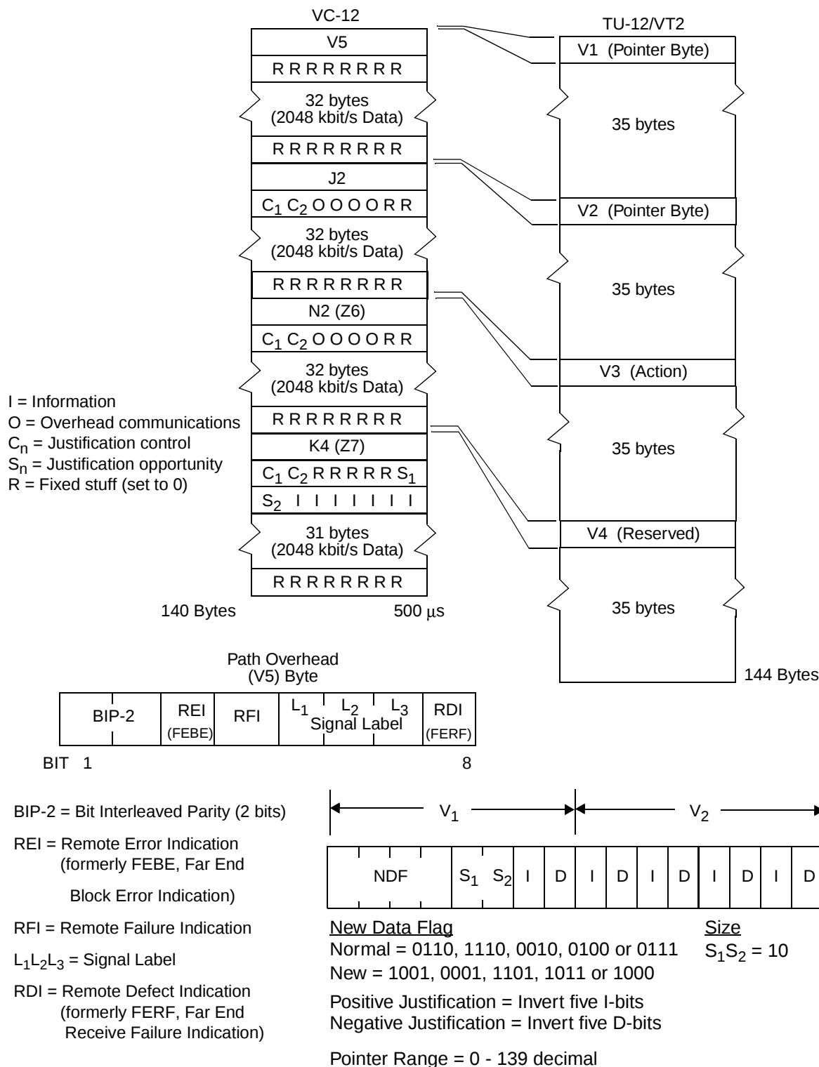
Figure 2. 2048 kbit/s Asynchronous Mapping
