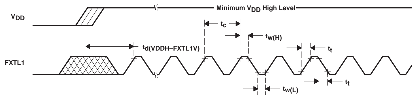
Figure 10. Crystal-Oscillator Timing
