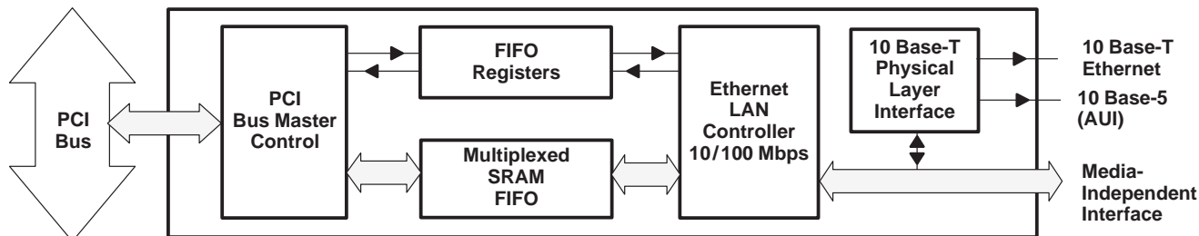
Figure 1. ThunderLAN Architecture
