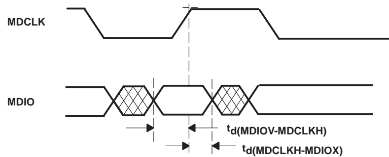
Figure 7. Management Data I/O Timing (Sourced by TNETE100PM)
