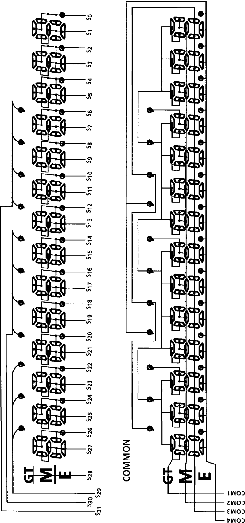
CONNECTION OF LCD (1) 14 DIGITS OF LCD SEGMENT
