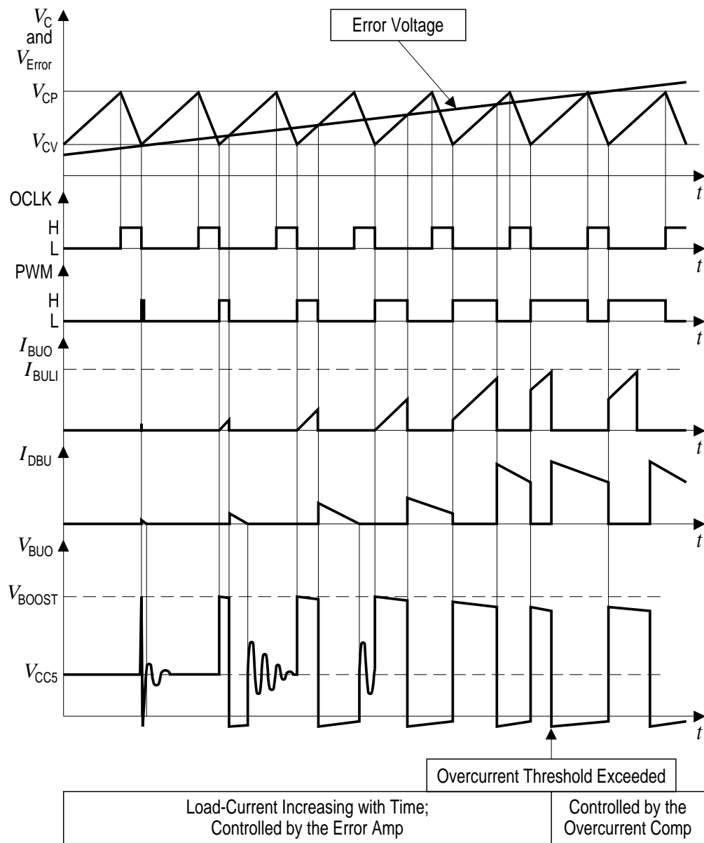
Figure 9 Most Important Waveforms of the Buck Converter Circuit
