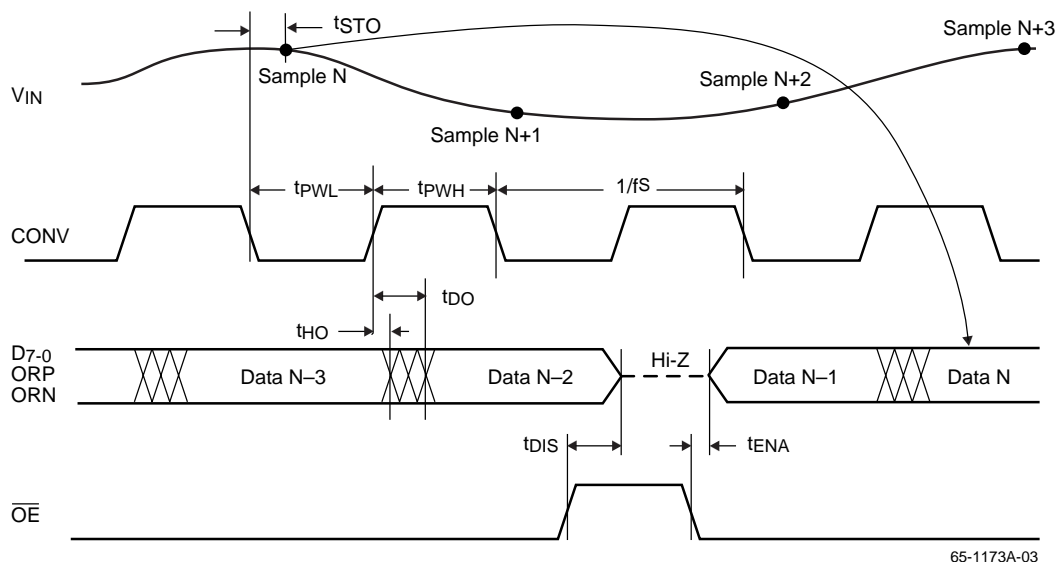
Figure 2. Conversion Timing
