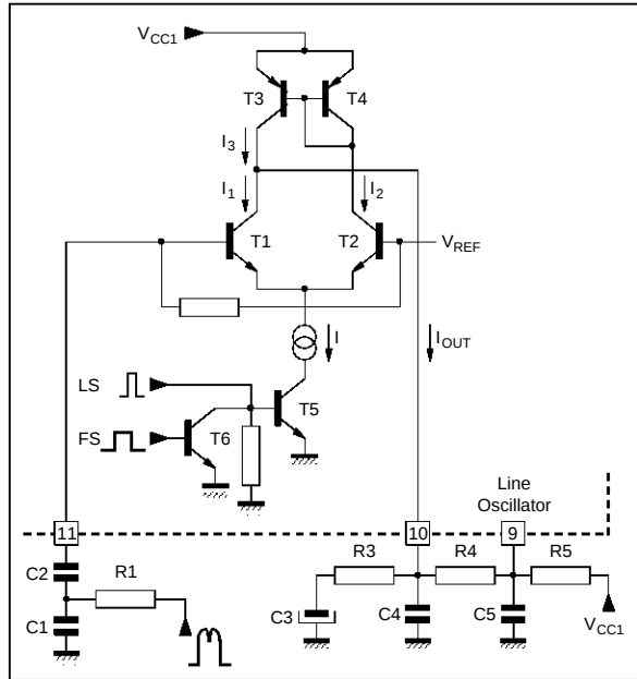
Figure 15 : Phase Comparator
