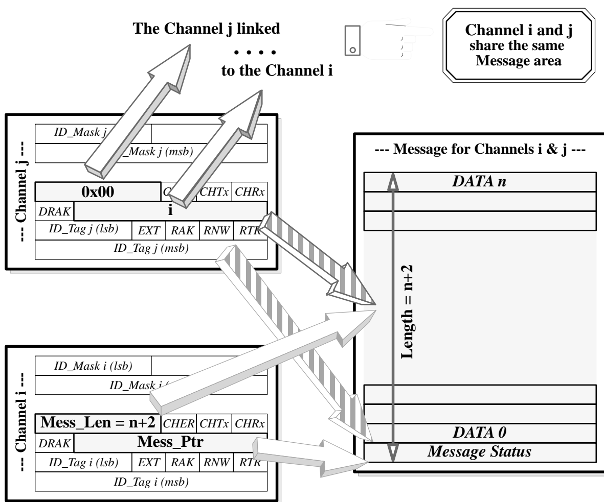
Figure 31. Linkage mechanism
