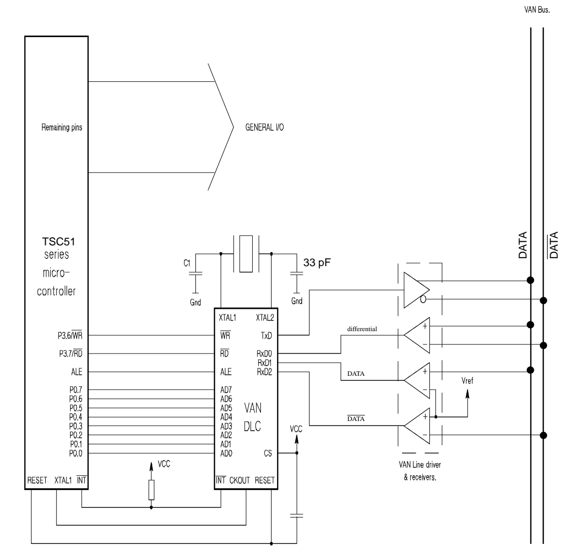
Figure 3. Typical Application
