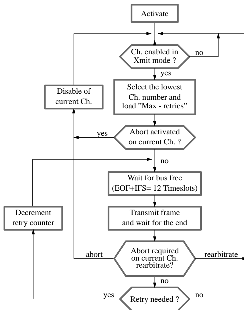
Figure 25. Transmit function
