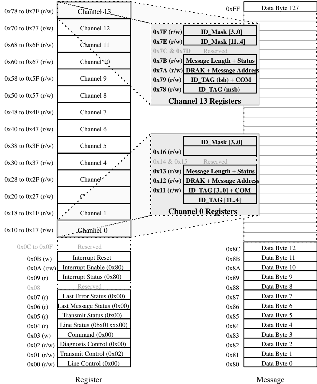
Figure 16. Memory Map.
