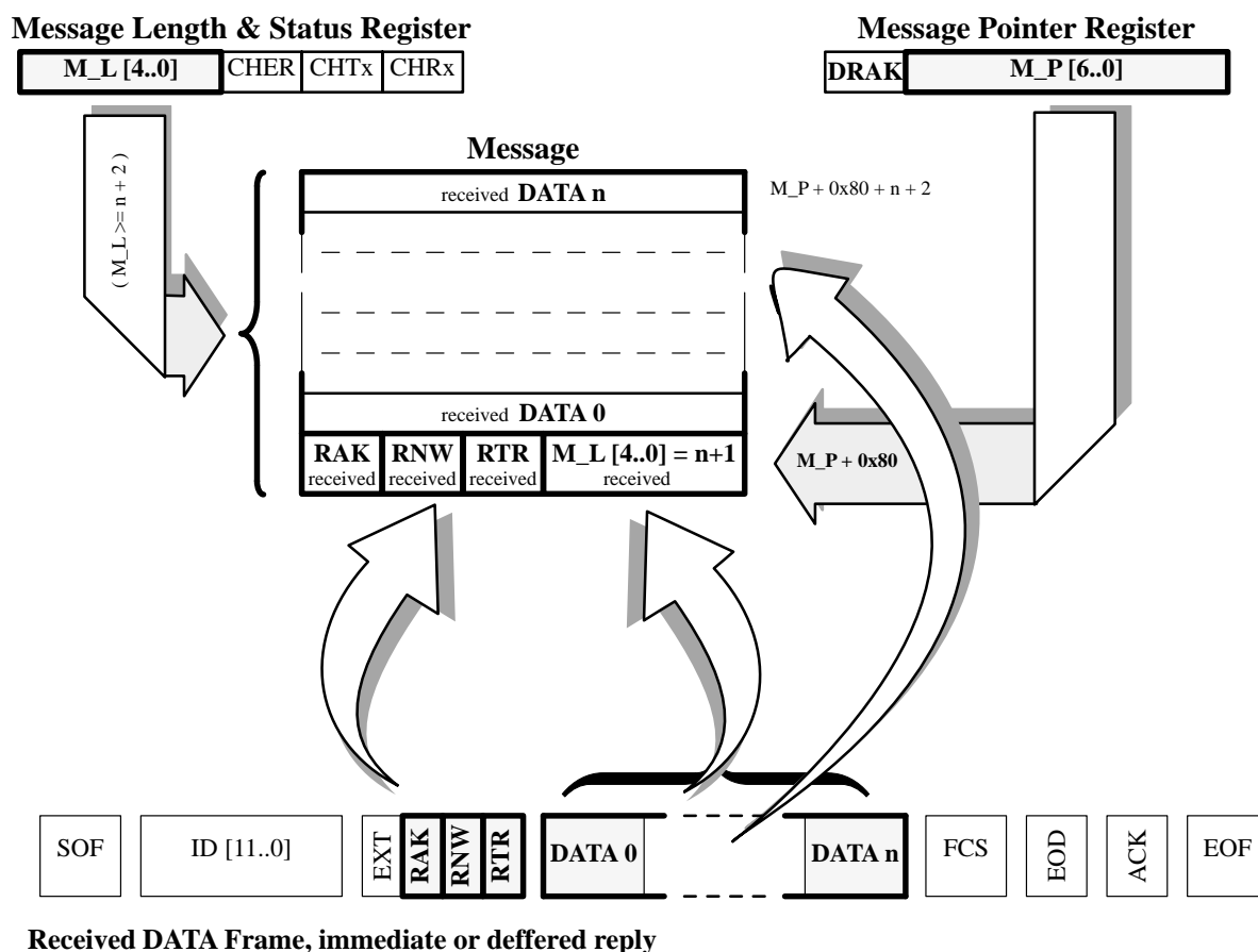
Figure 22. Message buffer structure for reception
