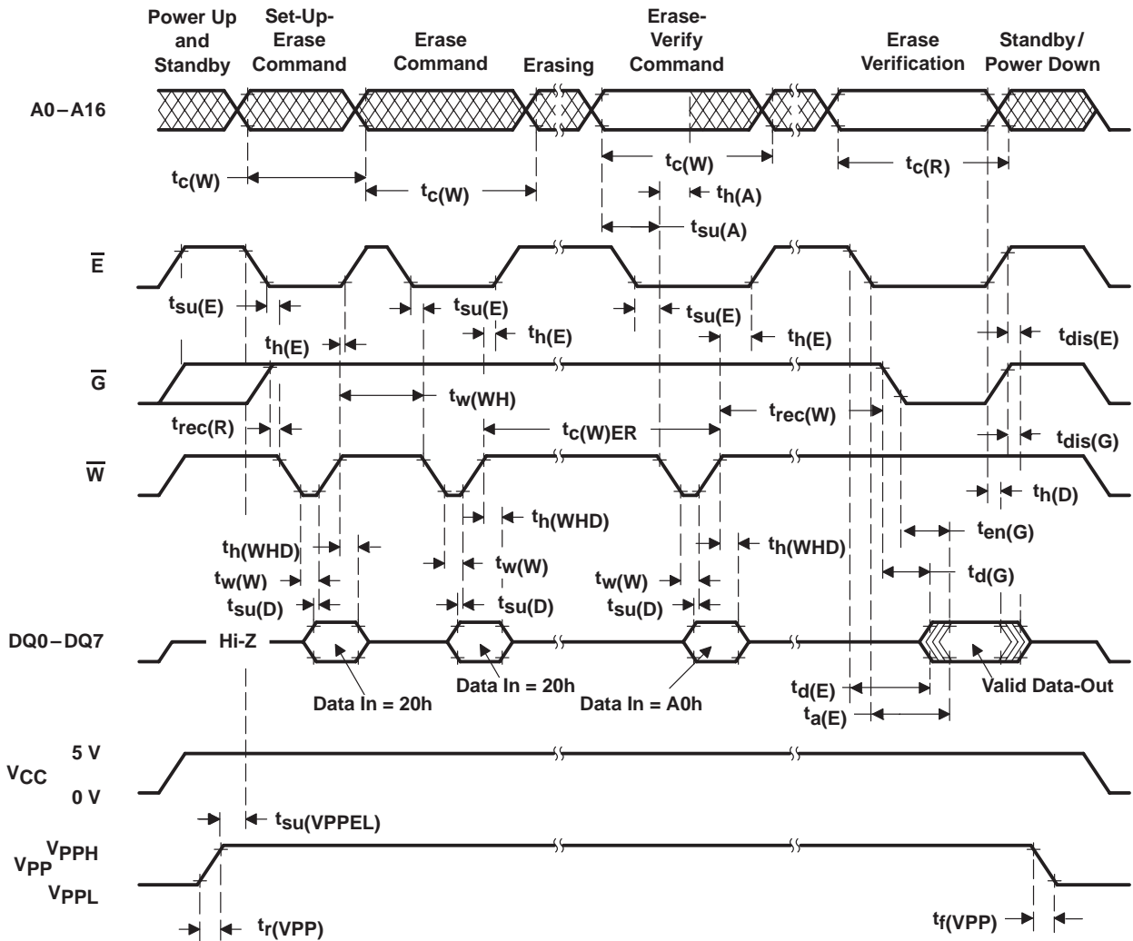
Figure 8. Flash-Erase-Cycle Timing
