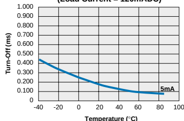
TS120 Typical Turn-Off vs. Temperature (Load Current = 120mA)
