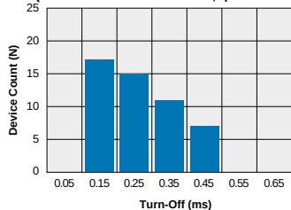
TS120 Typical Turn-Off Time (N=50 Ambient Temperature = 25°C) (Load Current = 120mA; I_F = 5\text{mA} )
