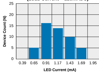
TS120 Typical I_F for Switch Operation (N=50 Ambient Temperature = 25°C) (Load Current = 120mA)
