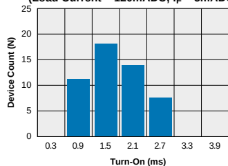
TS120 Typical Turn-On Time (N=50 Ambient Temperature = 25°C) (Load Current = 120mA; I_F = 5\text{mA} )
