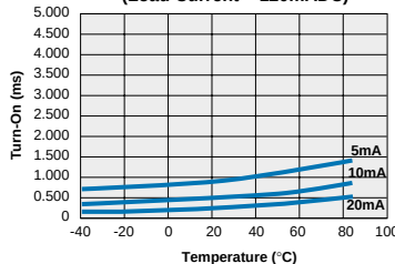
TS120 Typical Turn-On vs. Temperature (Load Current = 120mA)
