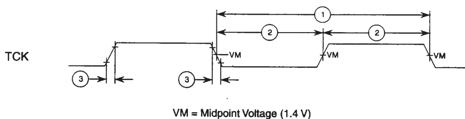
Figure 9 : Clock input timing diagram
