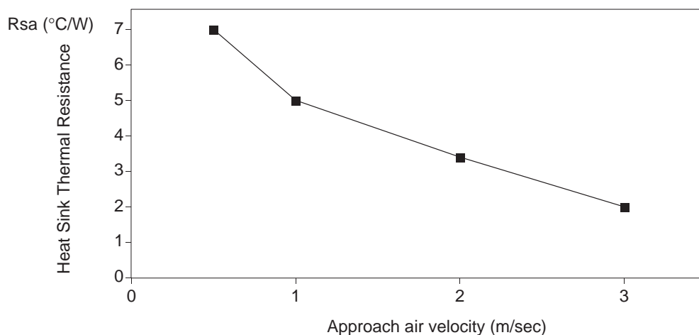
Figure 4 : CBGA thermal management example
