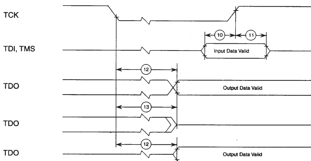
Figure 12 : Test access port timing diagram
