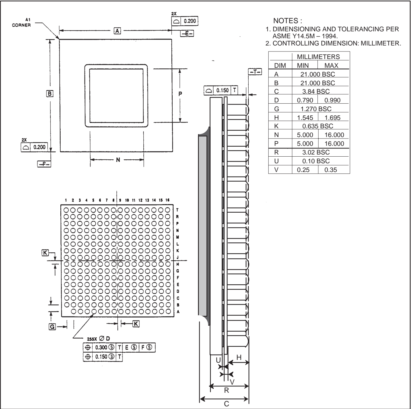
Figure 16 : Mechanical dimensions and bottom surface nomenclature of the CI-CGA package
