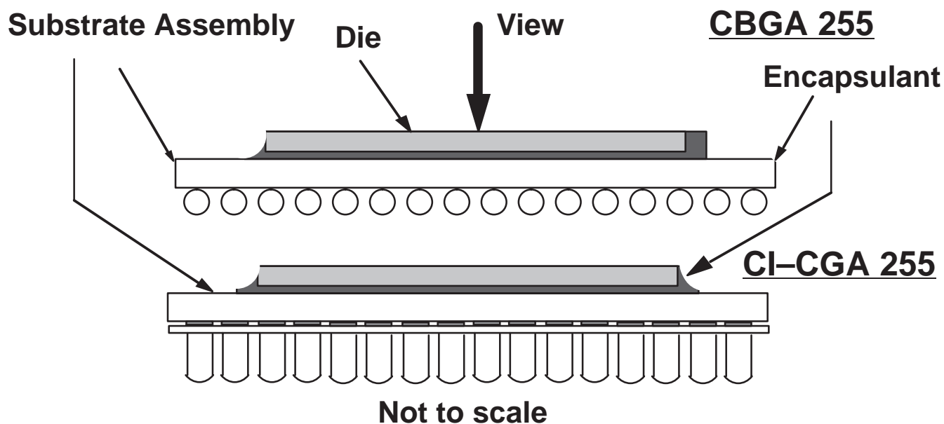
Figure 2 : CBGA 255 and CI-CGA 255 Top view
