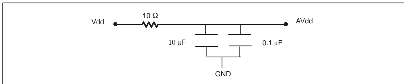
Figure 17 : PLL Power Supply Filter Circuit
