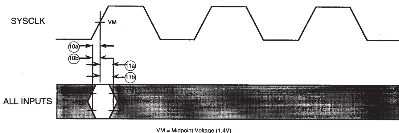
Figure 8 : Input timing diagram
