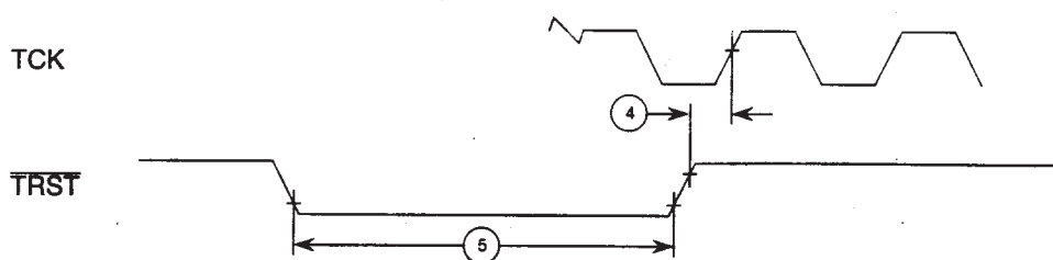
Figure 12 : \overline{\text{TRST}} timing diagram
