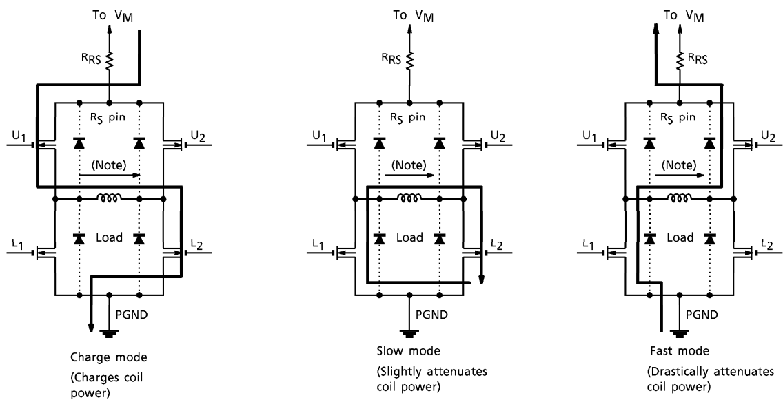
Output transistor operation functions
