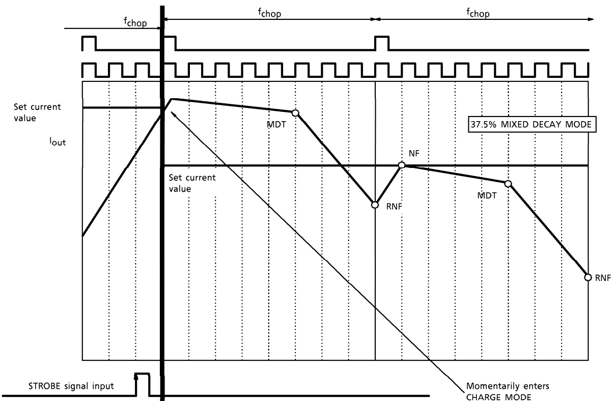
STROBE SIGNAL, INTERNAL CR CLK, AND OUTPUT CURRENT WAVEFORM (When STROBE signal is input in CHARGE MODE)
