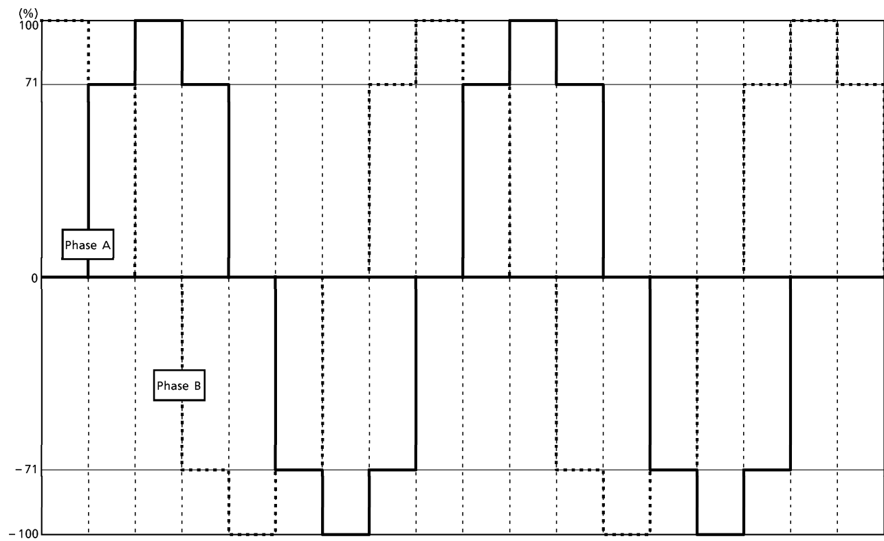
OUTPUT CURRENT WAVEFORM OF 1-2 PHASE EXCITATION SINE WAVE (Typ.B)
