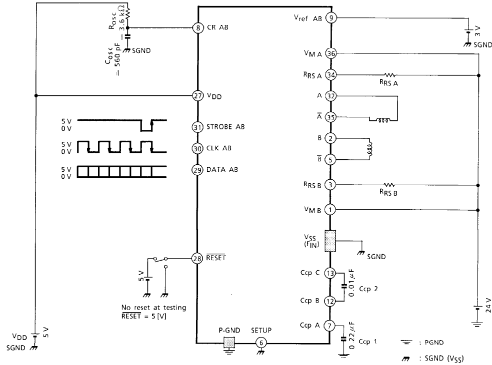
17. OSC-fast delay, OSC-charge delay (A/B unit only. C/D unit conforms to A/B unit.)
