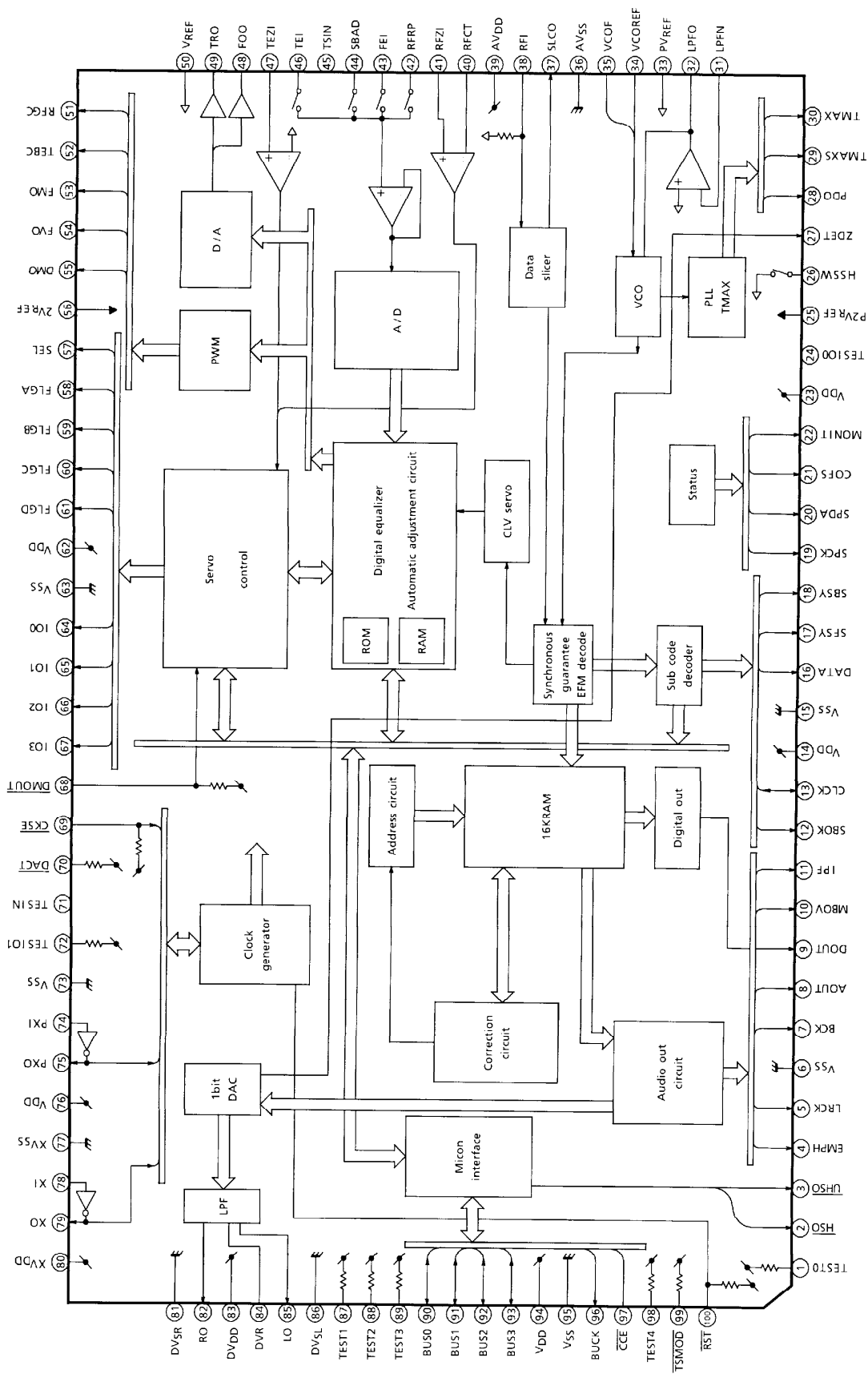
BLOCK DIAGRAM (Top view)
