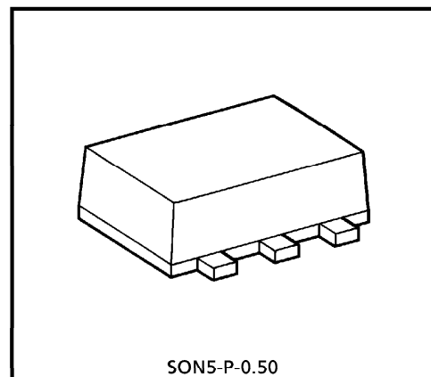
SON5-P-0.50
