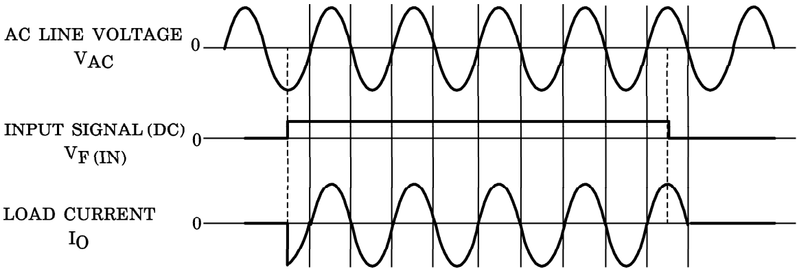
Fig.1 SWITCHING WAVEFORM
