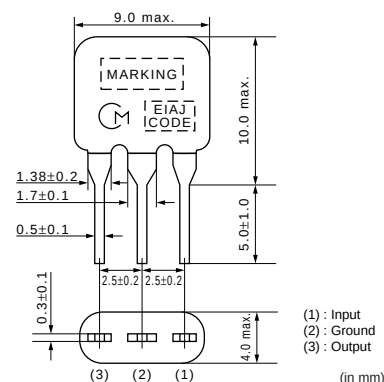
SFELA10M7JAXE-B0
