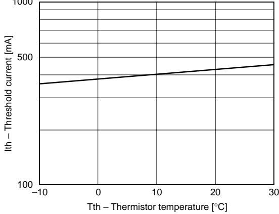
Threshold current vs. Temperature characteristics
