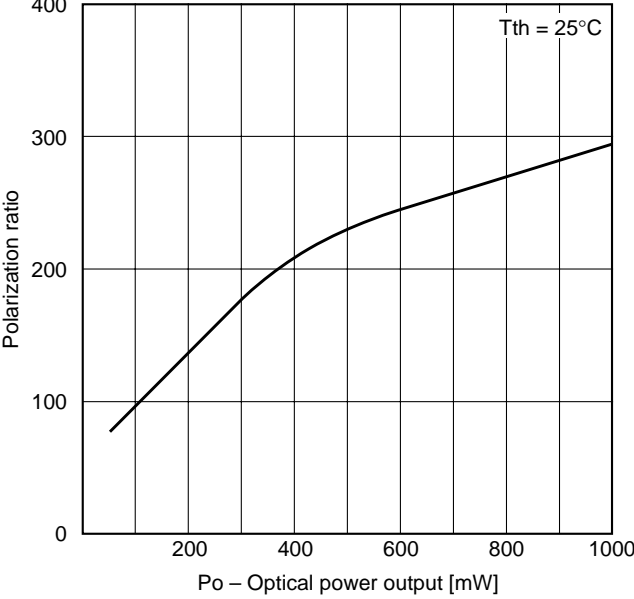
Power dependence of polarization ratio
