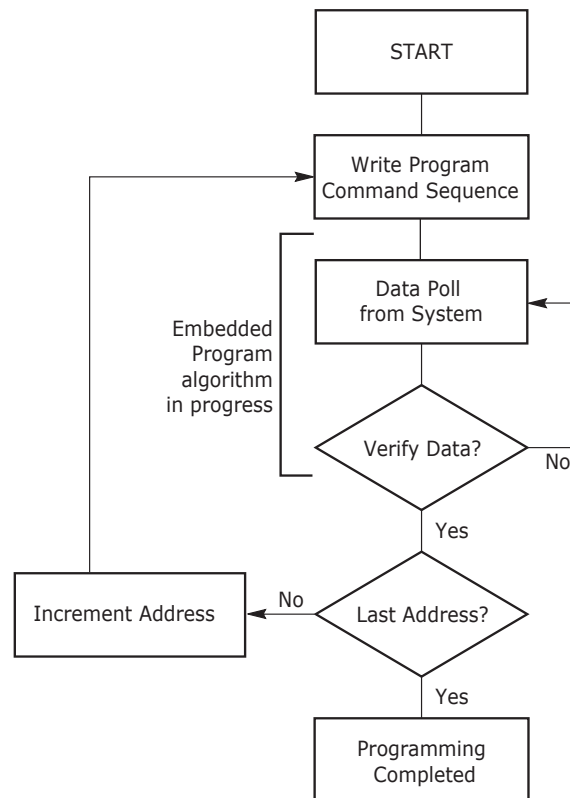
Figure 4. Program Operation
