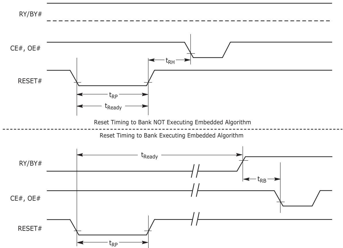
Figure I9. RESET# Timings
