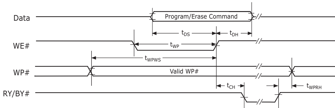
Figure 20. WP# Timing
