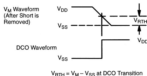
FIGURE 3. Reset Threshold
