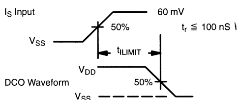
FIGURE 2. Current-Limit Comparator Response Time
