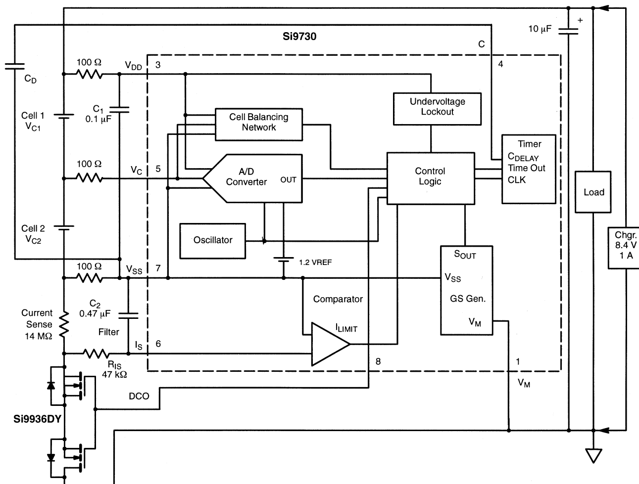
FIGURE 8. Typical 2-Cell Circuit
