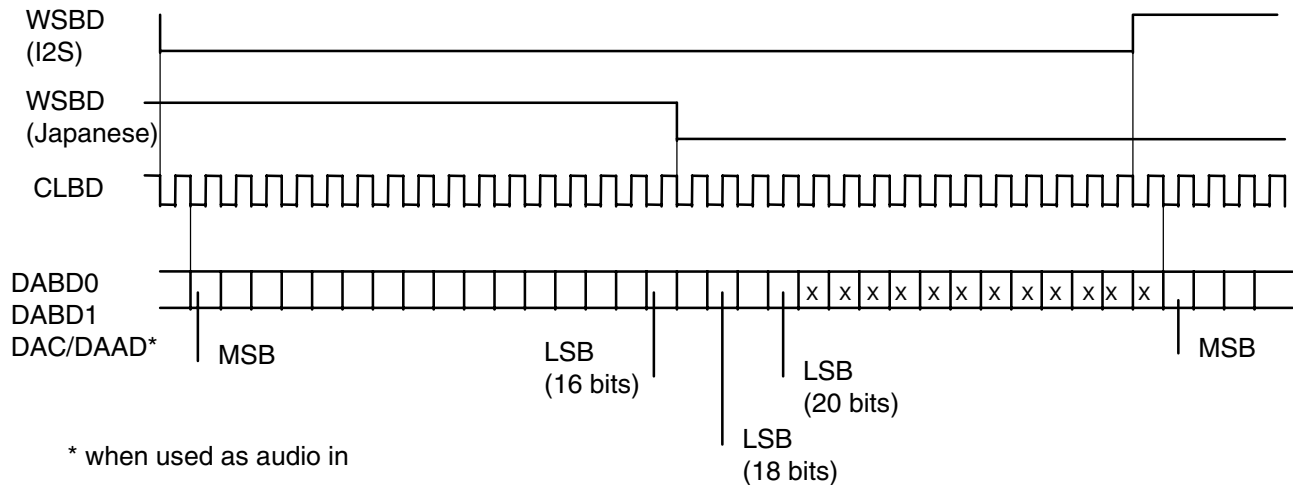
Figure 10. Digital Audio Frame Format
