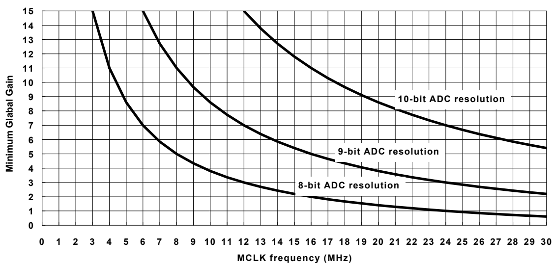
Figure 8. Recommended Minimum Global Gain Control Value
