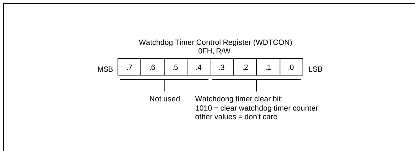
Figure 12-2. Watchdog Timer Control Register (WDTCN)
