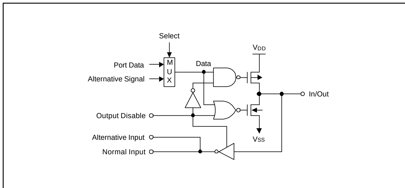
Figure 1-7. Pin Circuit Type 1 (Port 0, P1.0-P1.4, P6.0-P6.5, and Port 7)
