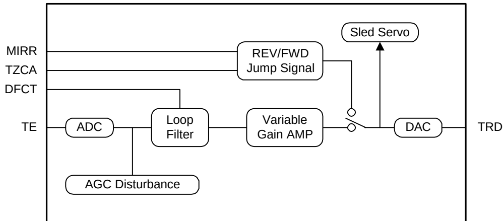
Tracking Servo Block Diagram
