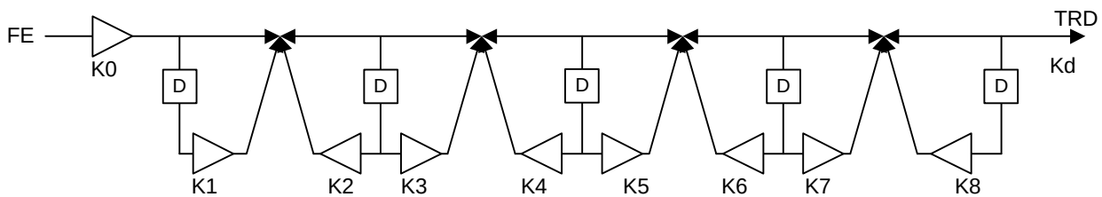
TRACKING LOOP FILTER
