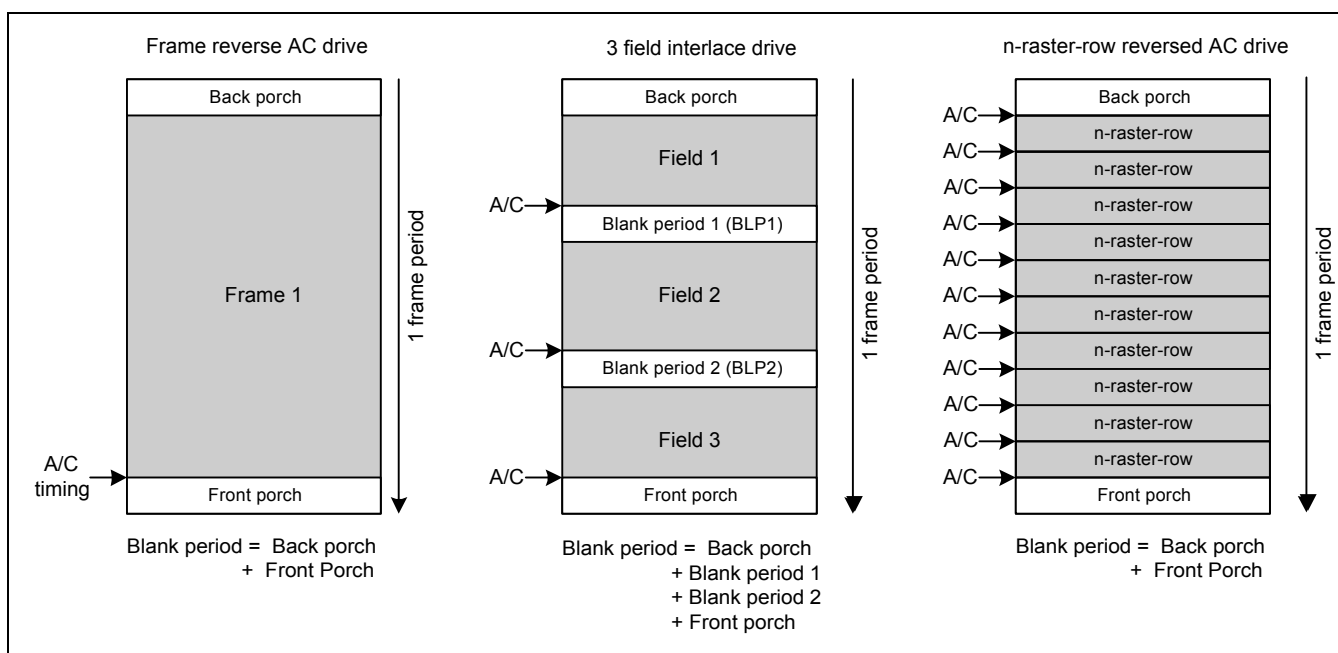
Figure 91. A/C timing
