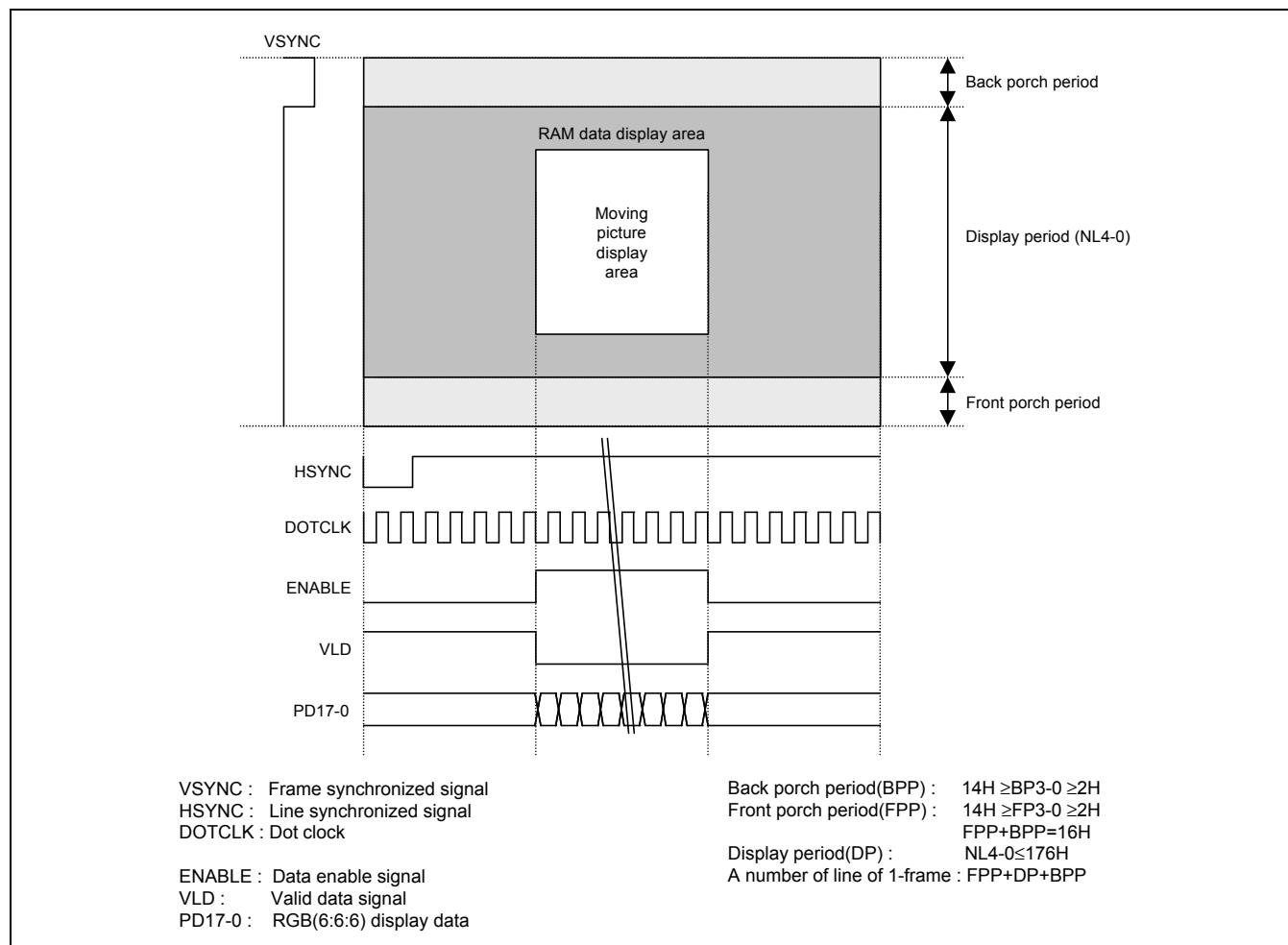
Figure 54. RGB Interface
