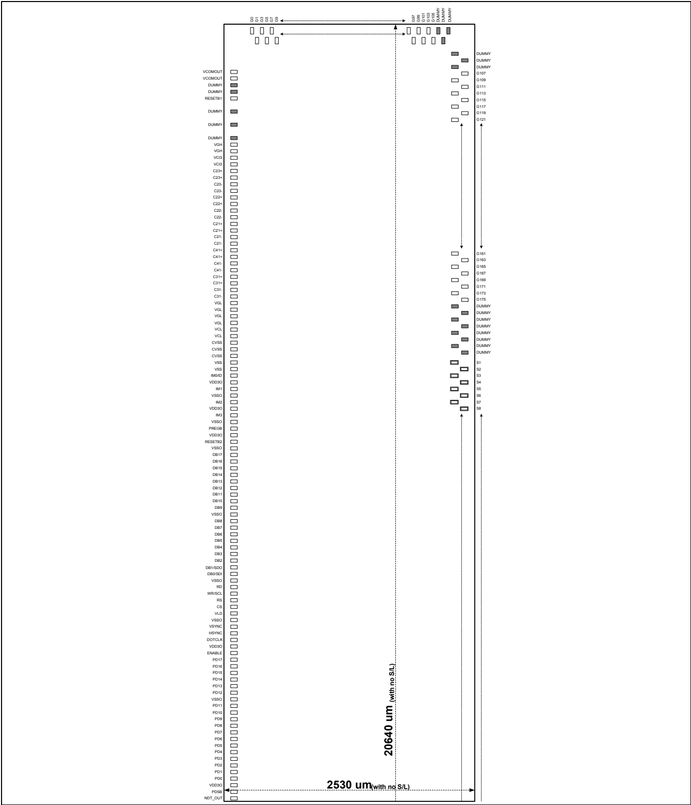
Figure 2. Pad Configuration
