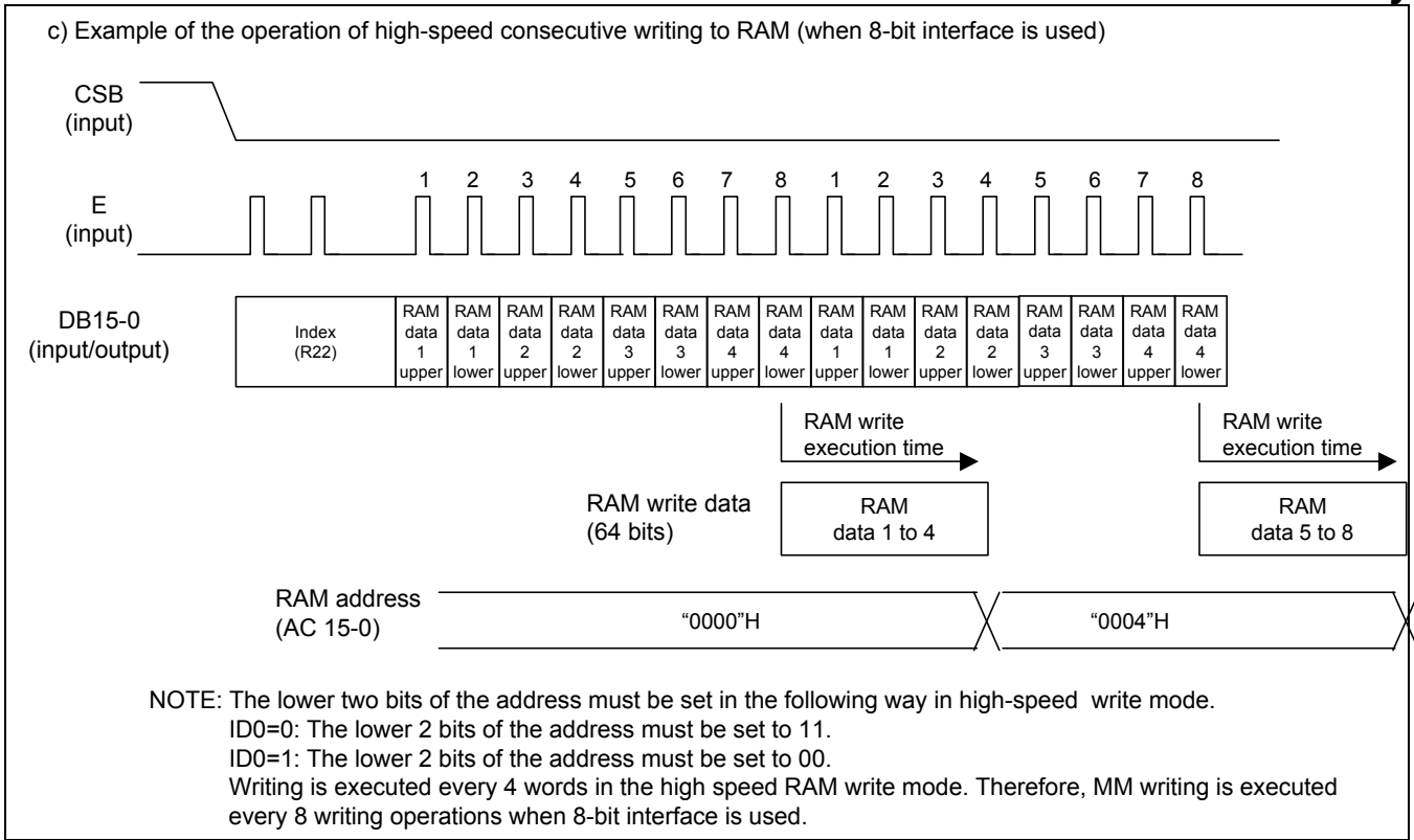
Figure 67. Example of the operation of high-speed consecutive writing to RAM (8-bit interface)
