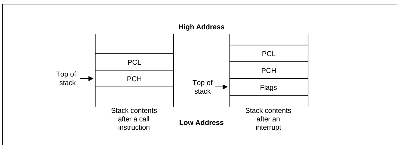
Figure 2-4. Stack Operations
