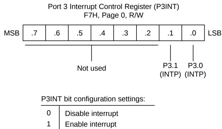
Figure 9-15. Port 3 Interrupt Control Register (P3INT)
