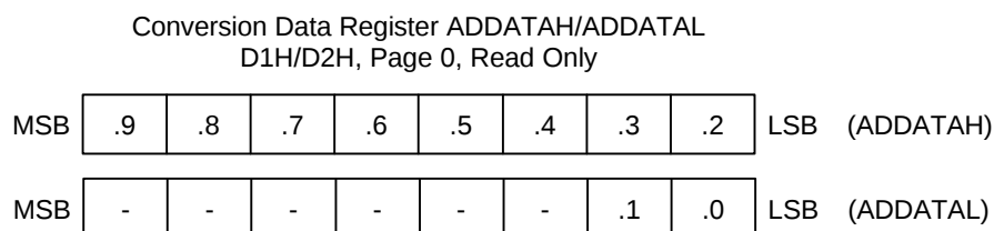
Figure 14-2. A/D Converter Data Register (ADDATAH/ADDATAL)
