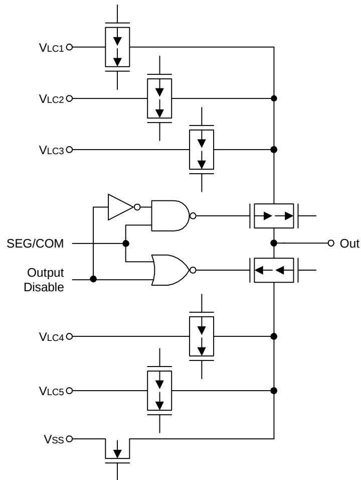
Figure 1-9. Pin Circuit Type H-23
