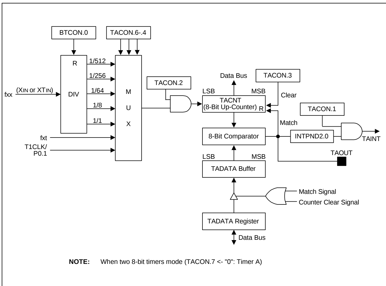
Figure 11-5. Timer A Block Diagram(Two 8-bit Timers Mode)
