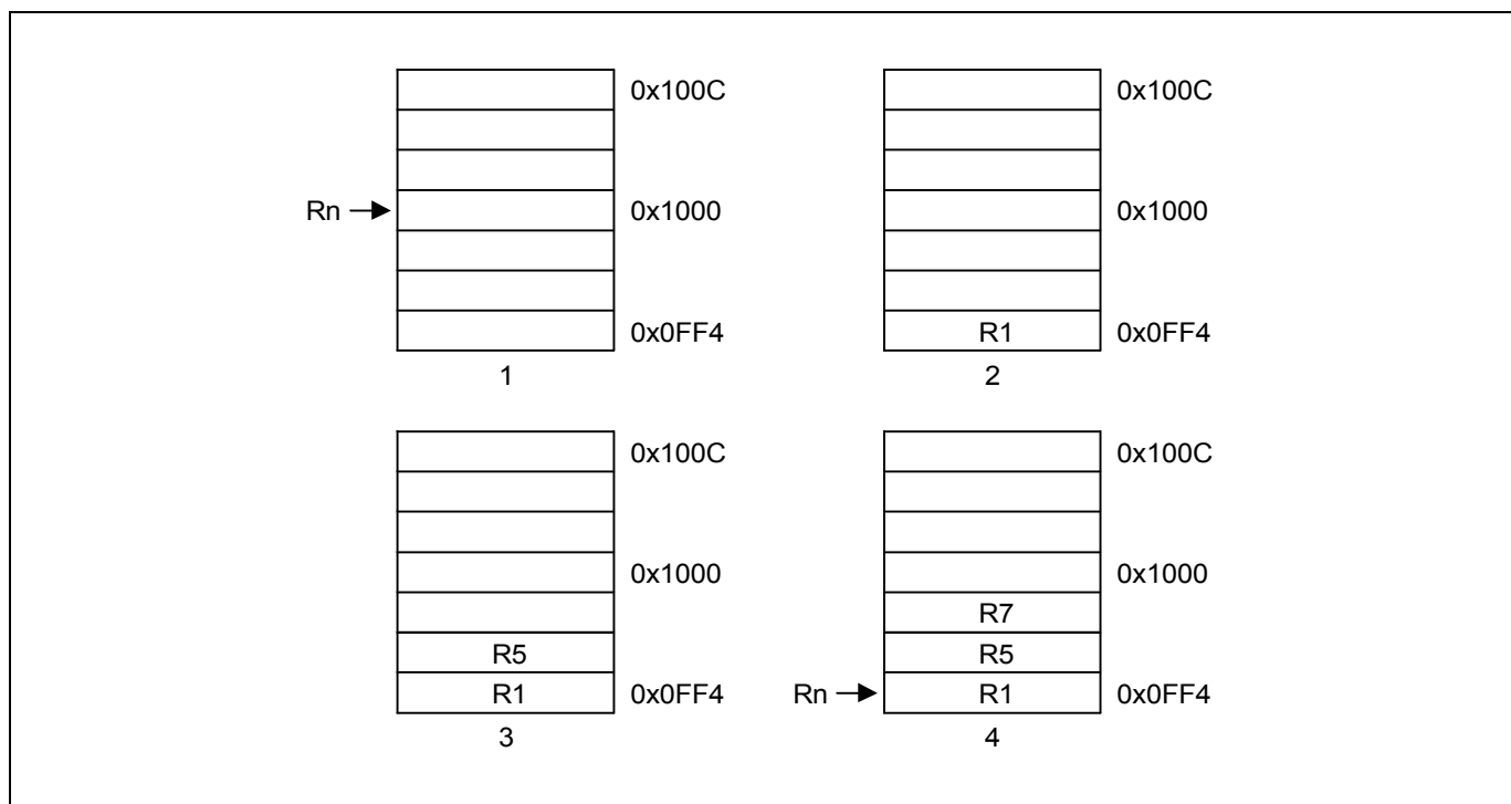
Figure 3-22. Pre-Decrement Addressing
