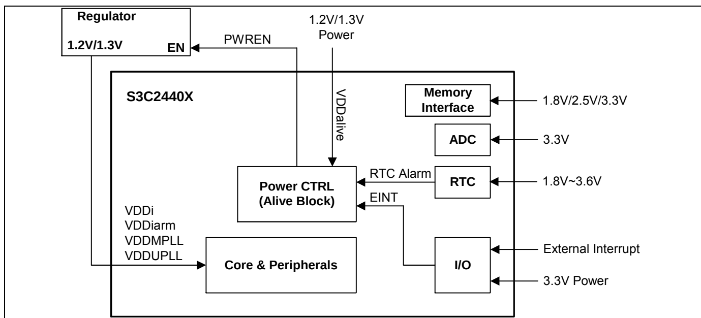
Figure 7-12. SLEEP Mode
