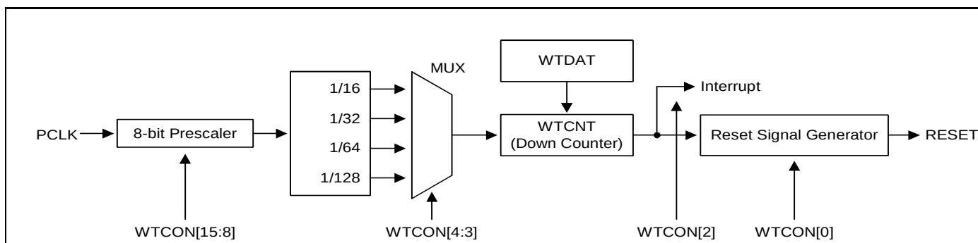
Figure 18-1. Watchdog Timer Block Diagram
