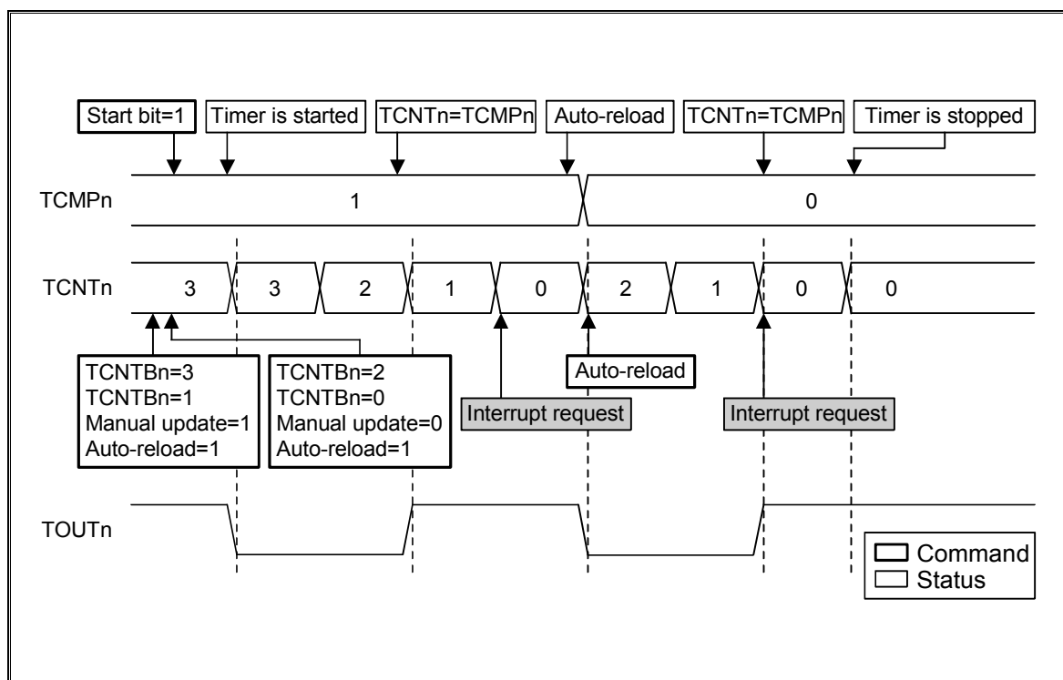
Figure 10-2. Timer Operations
