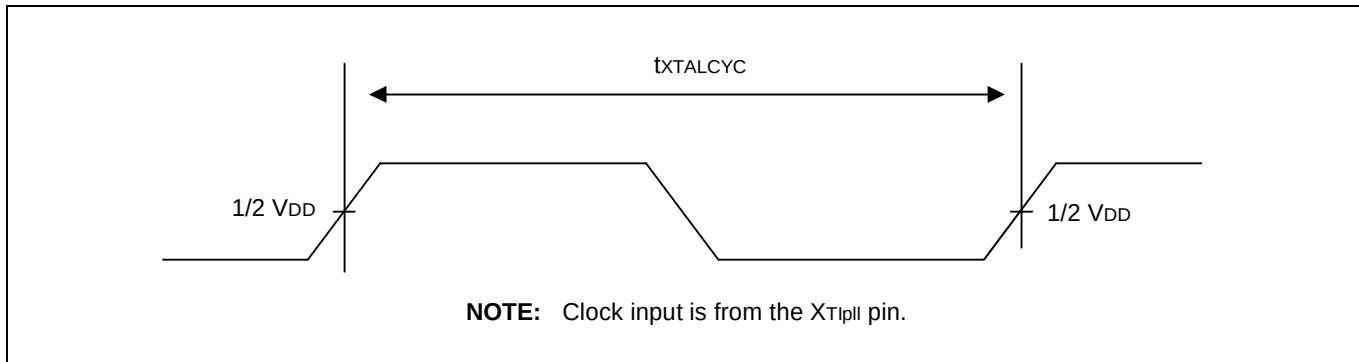
Figure 27-2 XTIpII Clock Timing Diagram
