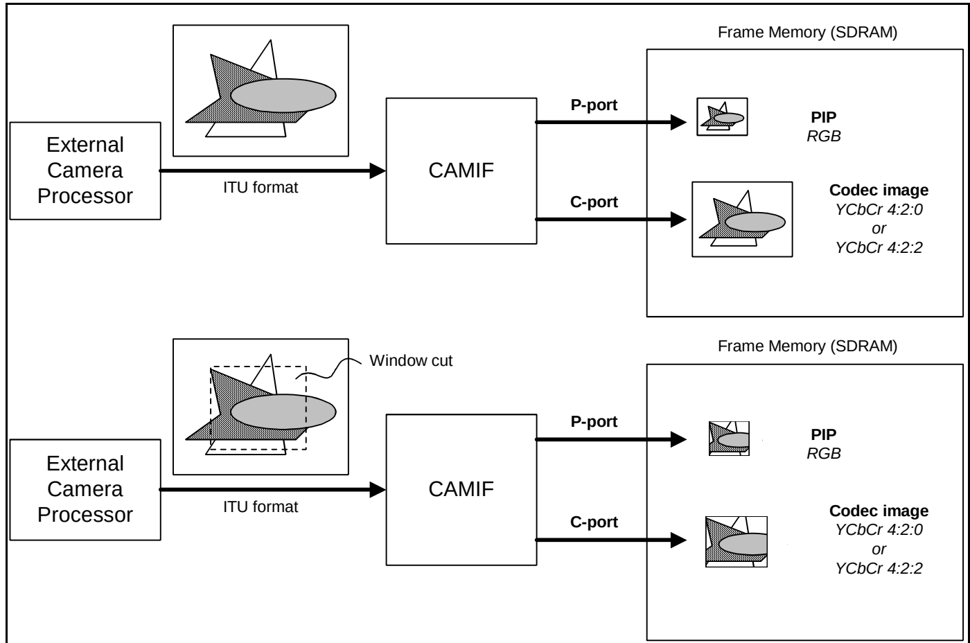
Figure 23-4 Two DMA Ports
