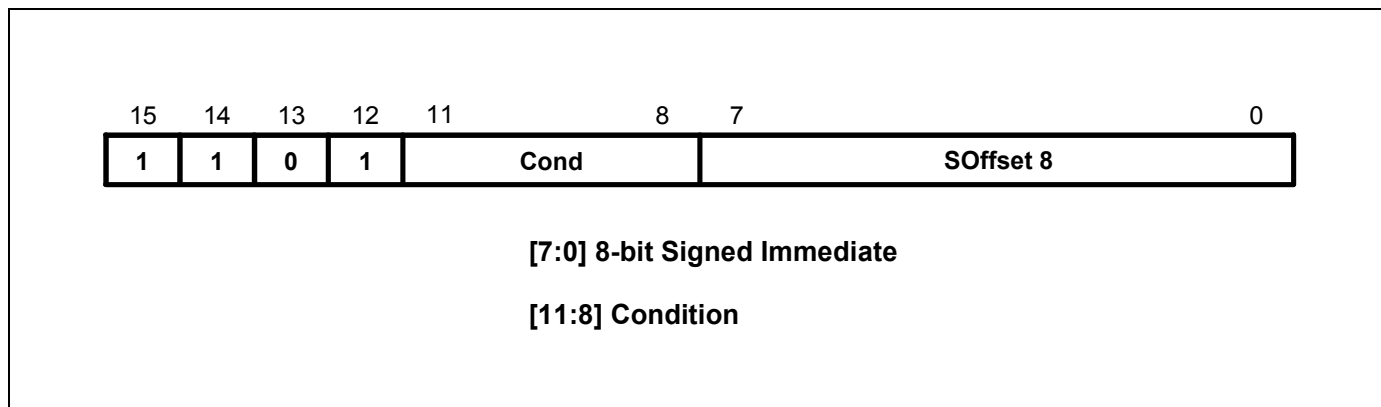
Figure 4-17. Format 16
