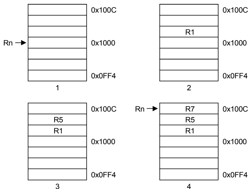
Figure 3-20. Pre-Increment Addressing
