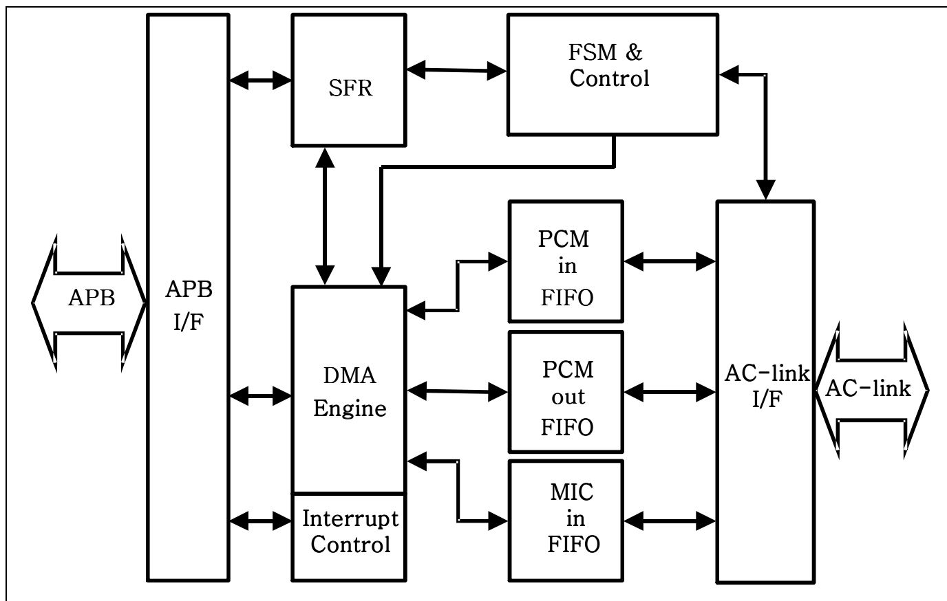
Figure 24-1 AC97 Block Diagram
