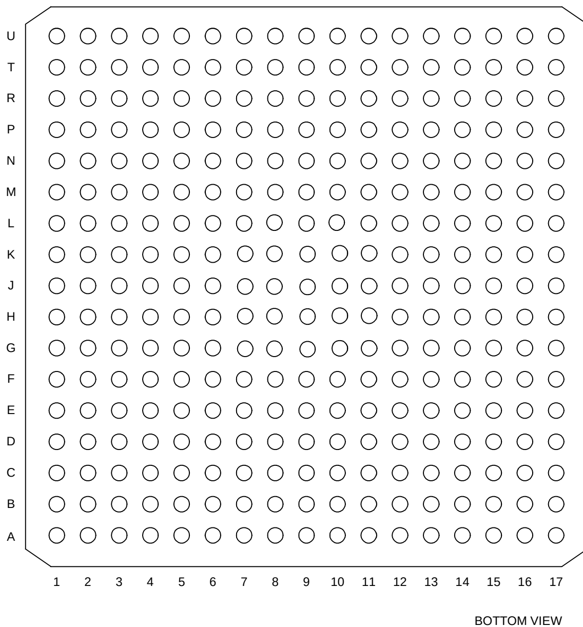
Figure 1-2. S3C2440A Pin Assignments (289-FBGA)
