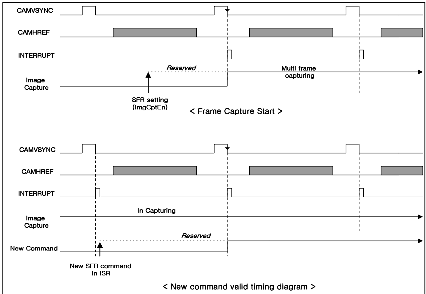
Figure 23-8 Timing Diagram for Register Setting
