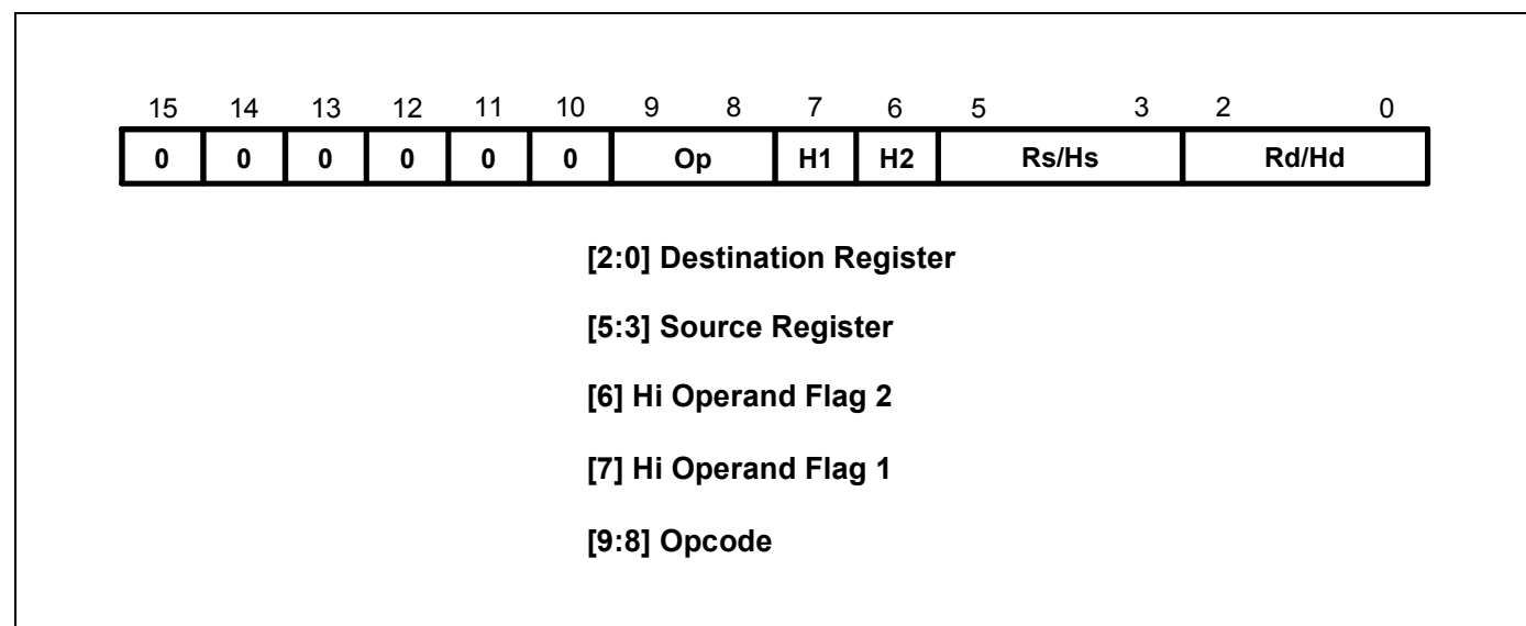
Figure 4-6. Format 5
