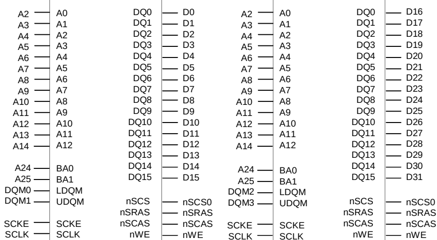
Figure 5-11. Memory Interface with 16-bit SDRAM (4Mx16x4Bank * 2ea)
