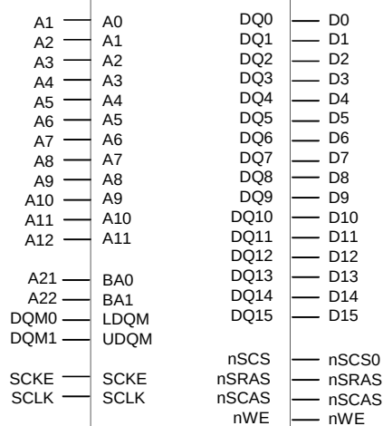
Figure 5-10. Memory Interface with 16-bit SDRAM (4Mx16, 4banks)
