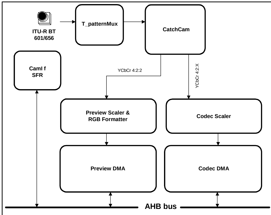
Figure 23-1 CAMIF Overview
