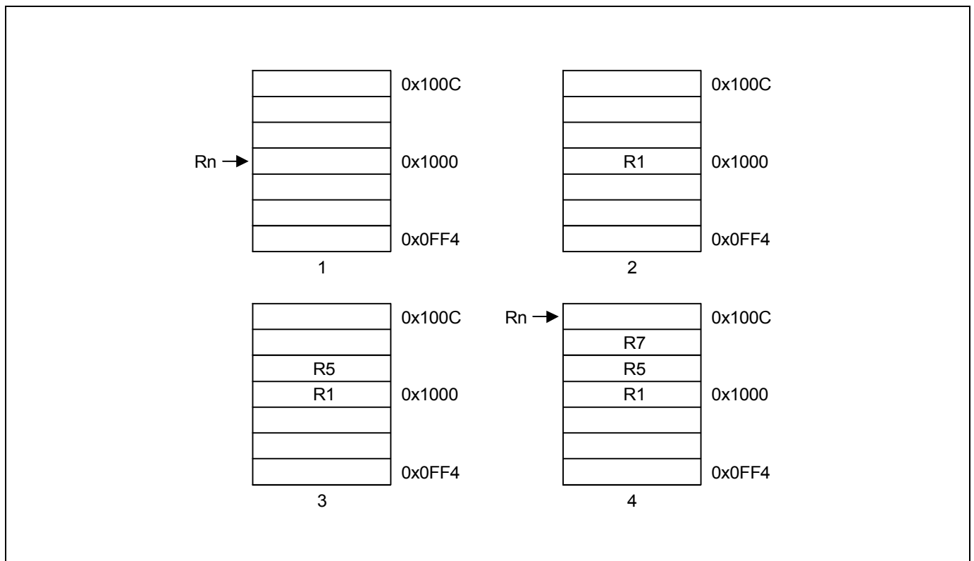
Figure 3-19. Post-Increment Addressing
