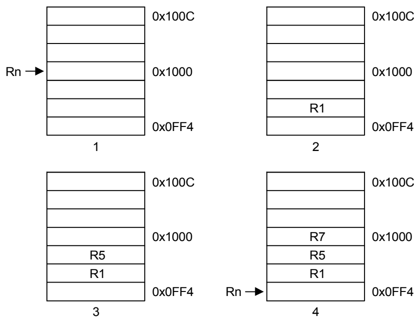
Figure 3-21. Post-Decrement Addressing
