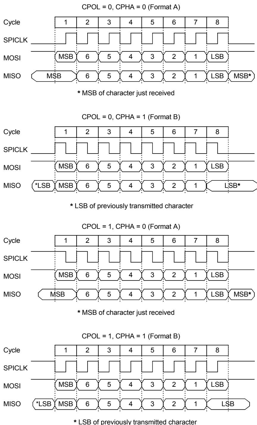
Figure 22-2 SPI Transfer Format
