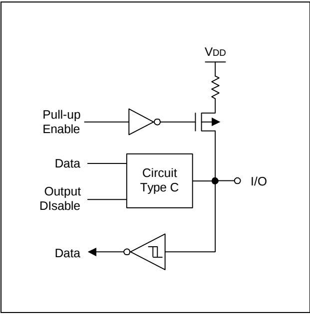
Figure 1-6. Pin Circuit Type D
