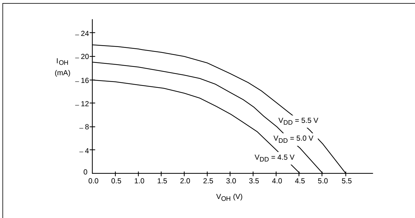
Figure 13-9. I_{OH} vs. V_{OH} (P1-P3, T_A = 25^\circ\text{C} )
