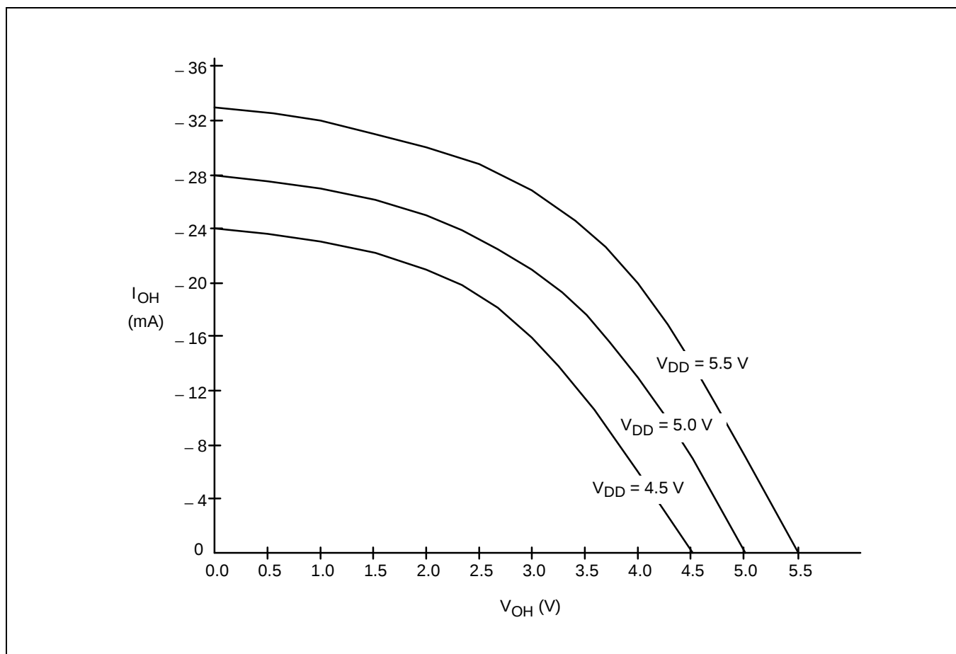
Figure 13-8. I_{OH} vs. V_{OH} (P0, T_A = 25^\circ\text{C} )
