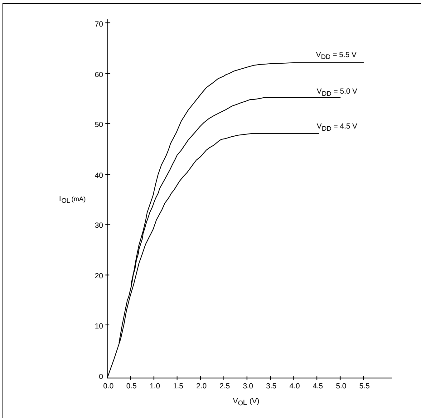
Figure 13-6. I_{OL} vs. V_{OL} (P0, T_A = 25^\circ\text{C} )
