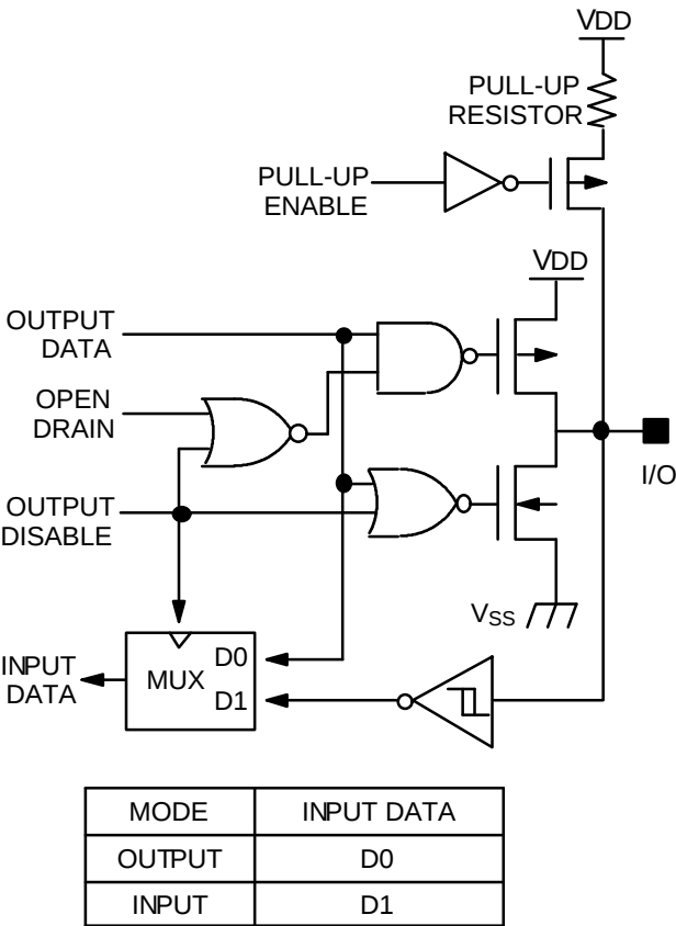
Figure 1-6. Pin Circuit Type D (Ports 2 and 4)
