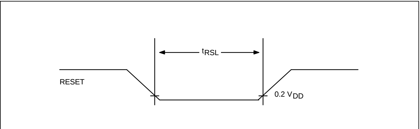
Figure 12-1. Input Timing for RESET
