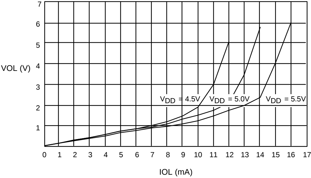
Figure 12-12. V_{OL} vs. I_{OL} (Port 0, 1, 2, and 4)
