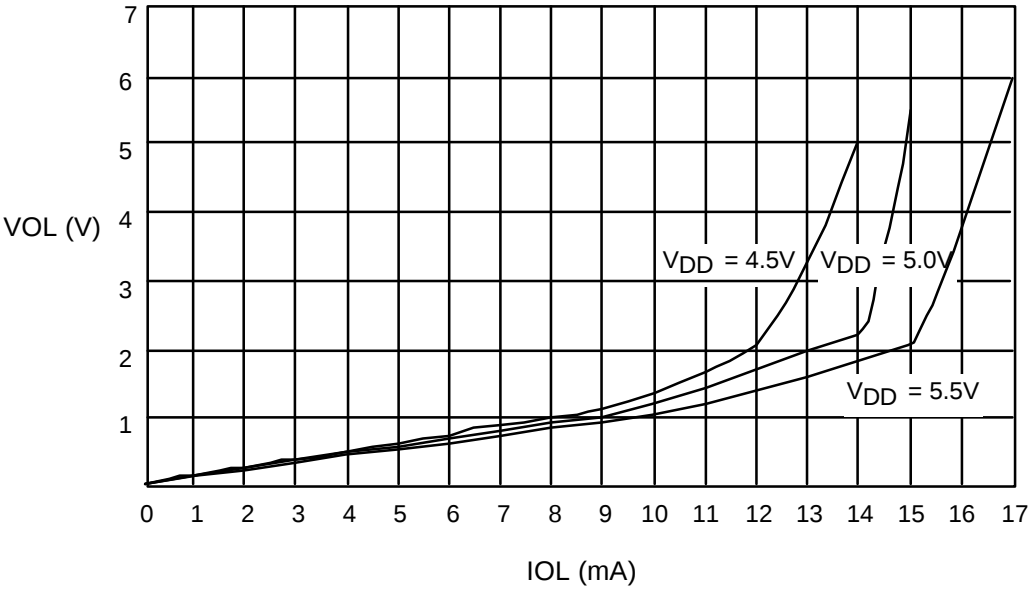
Figure 12-13. V_{OL} vs. I_{OL} (Port 3)
