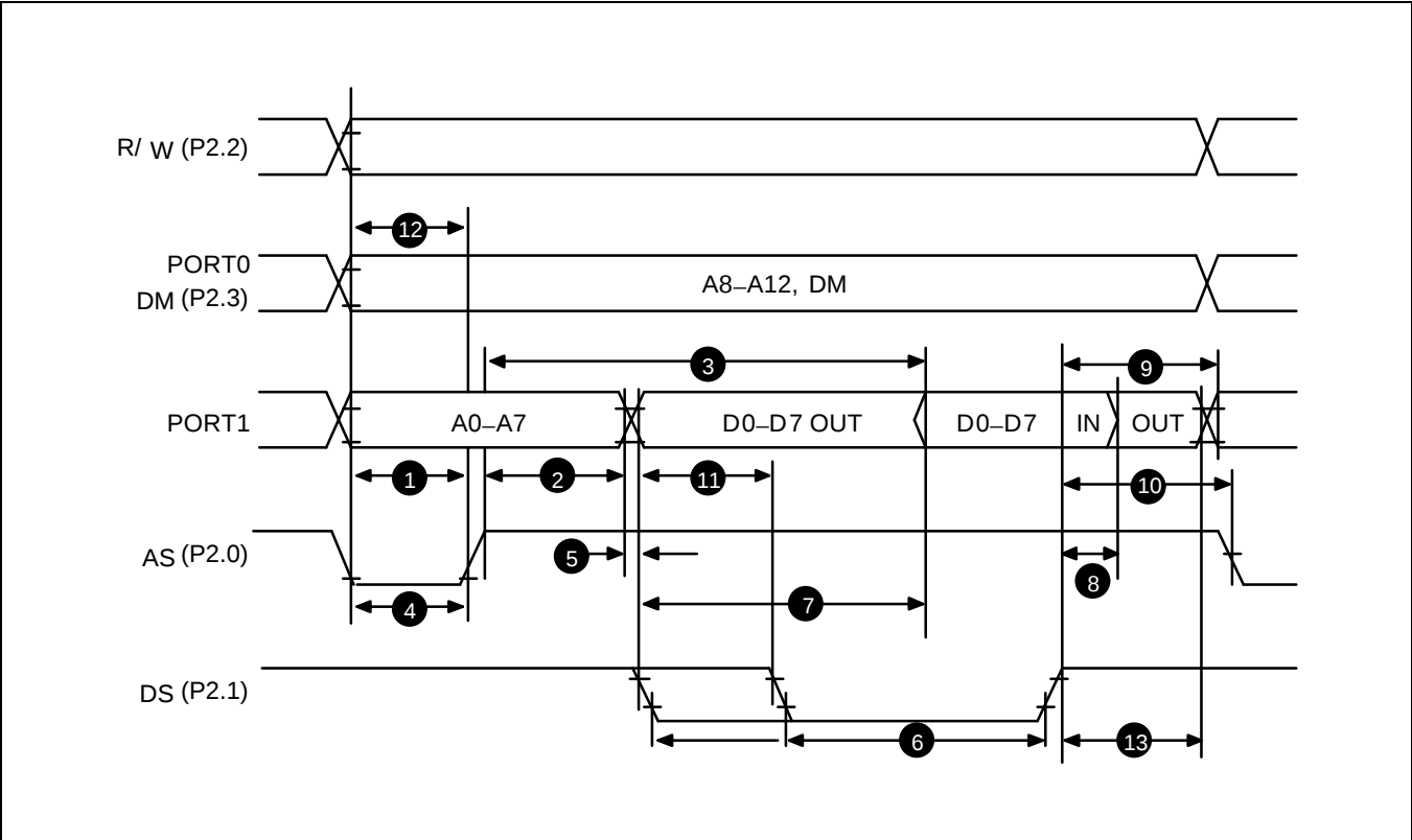
Figure 12-7. External Memory Read and Write Timing (See Table 12-8 for a description of each timing point.)
