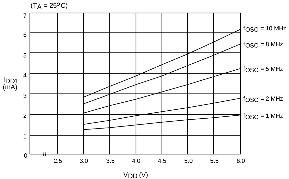
Figure 12-8. I_{DD1} vs. V_{DD}
