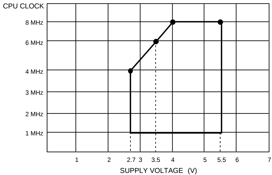
Figure 12-3. Operating Voltage Range (S3C9014/P9014)
