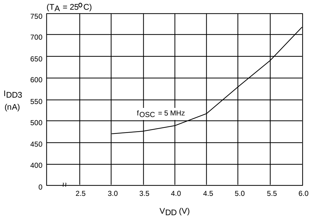
Figure 12-10. I_{DD3} vs. V_{DD}
