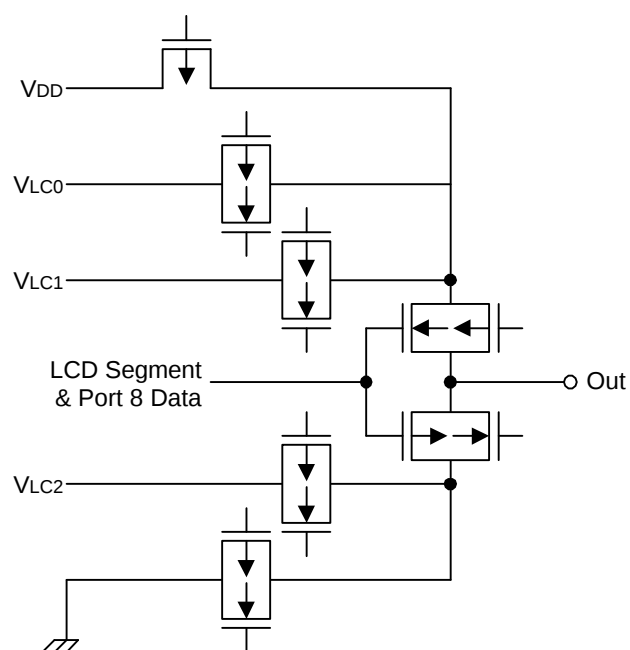
Figure 1-10. Pin Circuit Type H-16 (P8)
