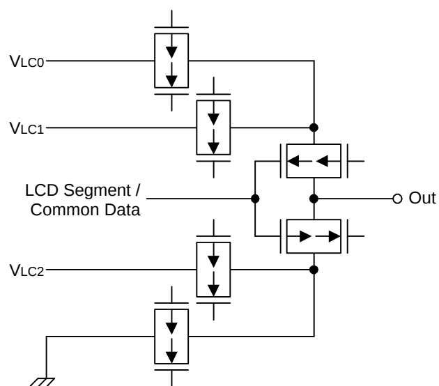
Figure 1-9. Pin Circuit Type H-15 (SEG/COM)
