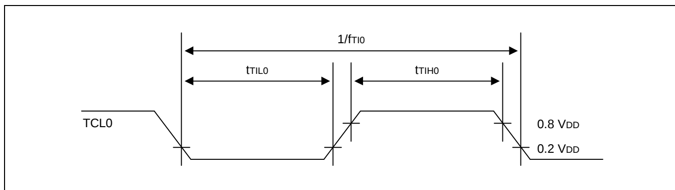
Figure 14-7. TCL0 Timing
