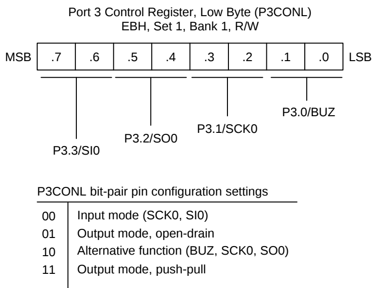
Figure 9-11. Port 3 Low-Byte Control Register (P3CONL)
