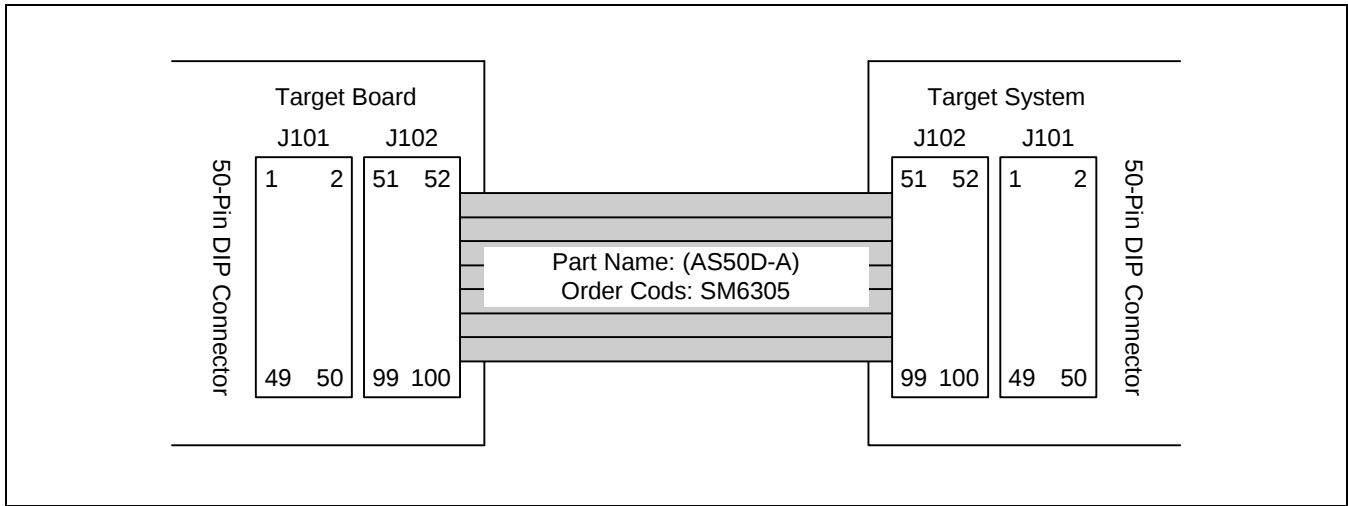
Figure 23-4. S3C830A/P830A Probe Adapter Cables for 100-QFP Package
