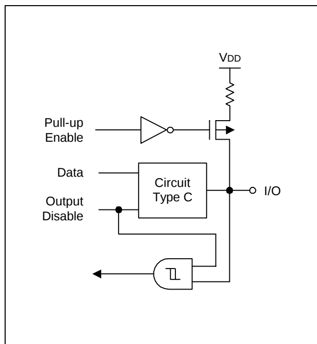
Figure 1-15. Pin Circuit Type D-4 (P2.4-P2.7)
