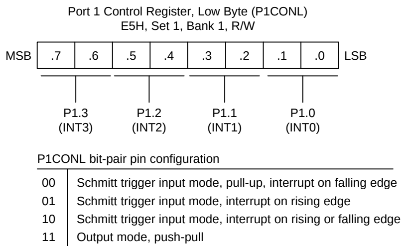
Figure 9-5. Port 1 Low-Byte Control Register (P1CONL)
