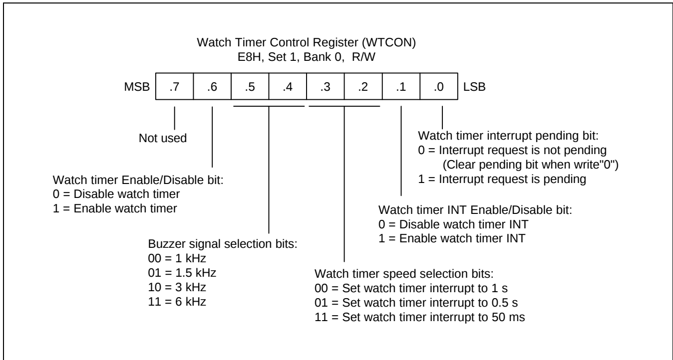
Figure 13-1. Watch Timer Control Register (WTCON)
