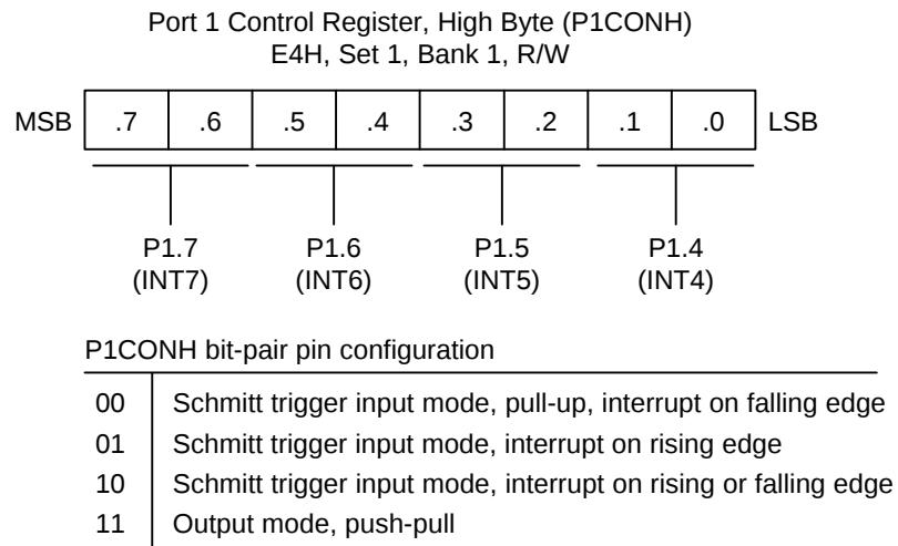
Figure 9-4. Port 1 High-Byte Control Register (P1CONH)
